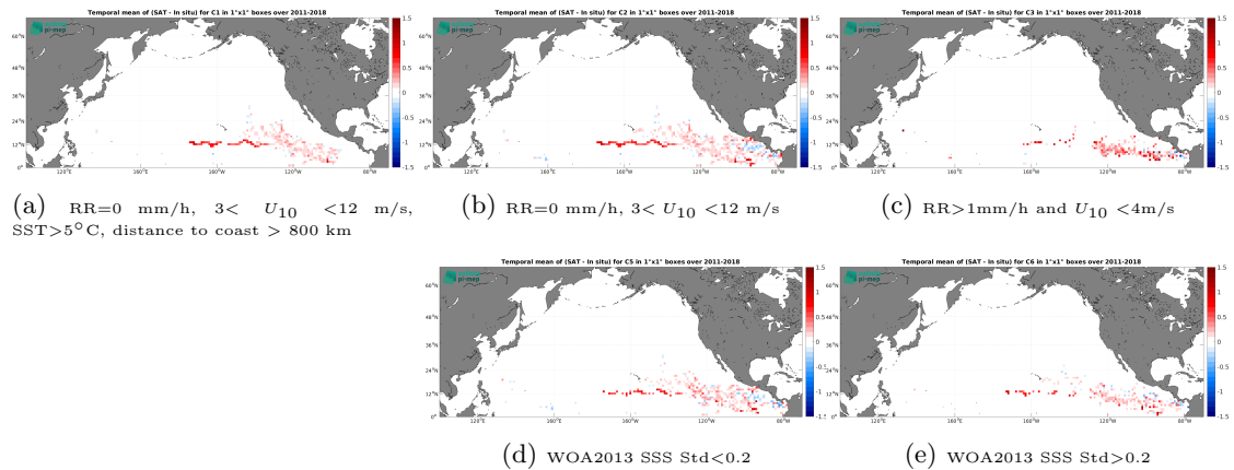
Figure 13: Temporal mean gridded over spatial boxes of size 1^\circ \times 1^\circ of \Delta SSS (CCI SSS L4 Merged-OI v4.41 - 7-day running (ESA) - Surface drifters) for 5 different subdatasets corresponding to:RR=0 mm/h, 3 < U_{10} < 12 m/s, SST >5^\circ C, distance to coast > 800 km (a), RR=0 mm/h, 3 < U_{10} < 12 m/s (b), RR >1 mm/h and U_{10} < 4 m/s (c), WOA2013 SSS Std <0.2 (d), WOA2013 SSS Std >0.2 (e).
