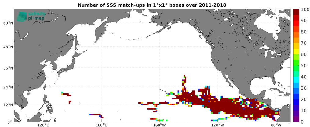
Figure 4: Number of SSS match-ups between Surface drifters SSS and the CCI SSS L4 Merged-OI v4.41 - 7-day running (ESA) SSS product for the North Pacific Ocean Pi-MEP region over 1^\circ \times 1^\circ boxes and for the full satellite product period.
