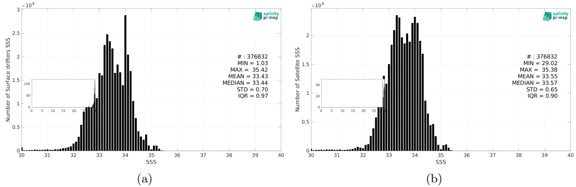
Figure 3: Histograms of SSS from Surface drifters (a) and CCI SSS L4 Merged-OI v4.41 - 7-day running (ESA) (b) considering all match-up pairs per bins of 0.1 over the North Pacific Ocean Pi-MEP region and for the full satellite product period.
