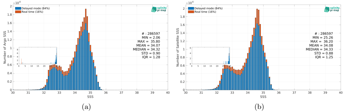
Figure 3: Histograms of SSS from Argo (a) and CCI SSS L4 Merged-OI v4.41 - 7-day running (ESA) (b) considering all match-up pairs per bins of 0.1 over the North Pacific Ocean Pi-MEP region and for the full satellite product period.
