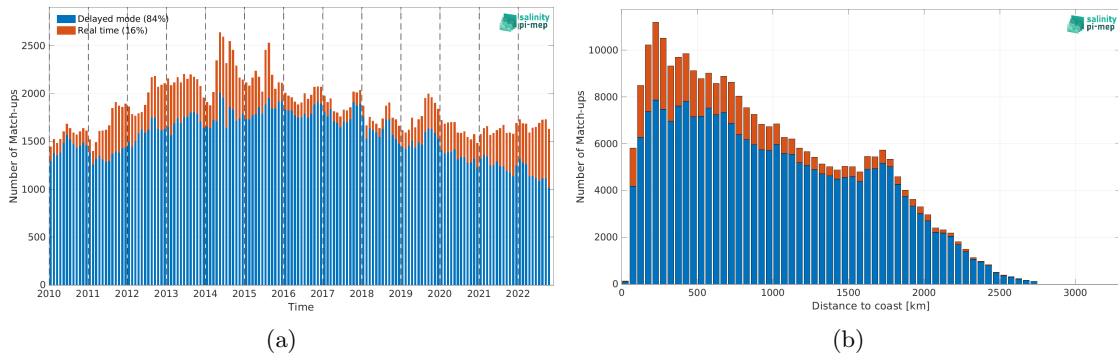
Figure 2: Number of match-ups between Argo and CCI SSS L4 Merged-OI v4.41 - 7-day running (ESA) SSS as a function of time (a) and as function of the distance to coast (b) over the North Pacific Ocean Pi-MEP region and for the full satellite product period.
