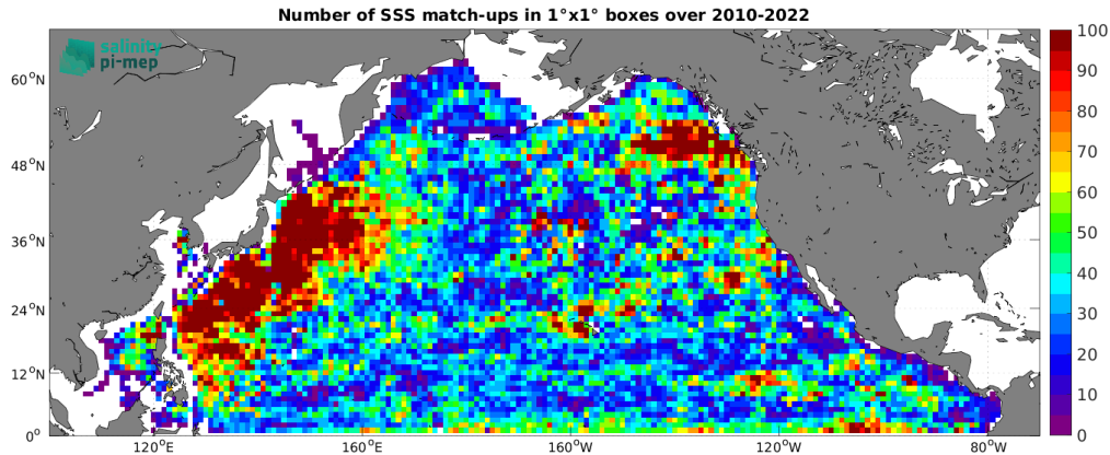
Figure 5: Number of SSS match-ups between Argo SSS and the CCI SSS L4 Merged-OI v4.41 - 7-day running (ESA) SSS product for the North Pacific Ocean Pi-MEP region over 1^\circ \times 1^\circ boxes and for the full satellite product period.
