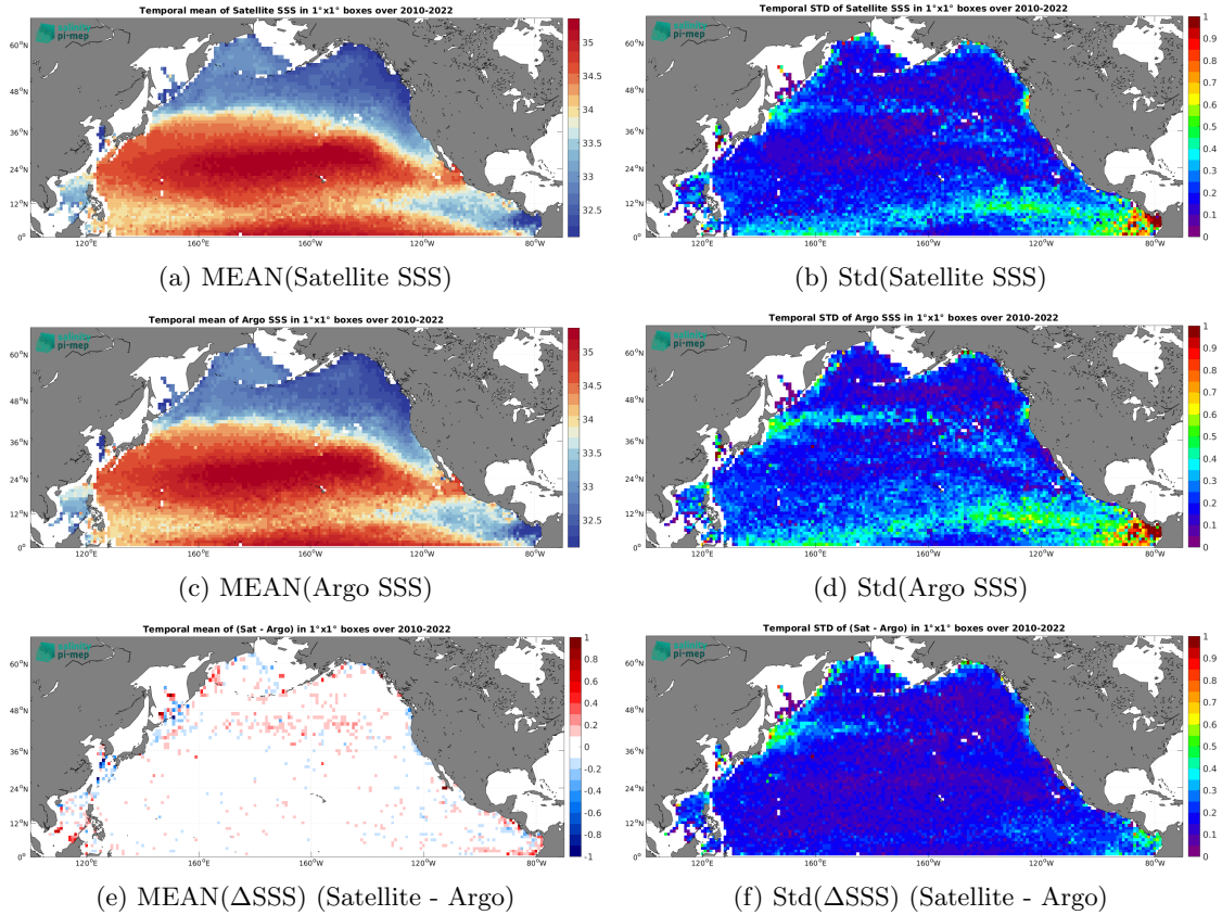
Figure 7: Temporal mean (left) and Std (right) of SSS from CCI SSS L4 Merged-OI v4.41 - 7-day running (ESA) (top), Argo (middle), and of \Delta\text{SSS} (Satellite - Argo). Only match-up pairs are used to generate these maps.
