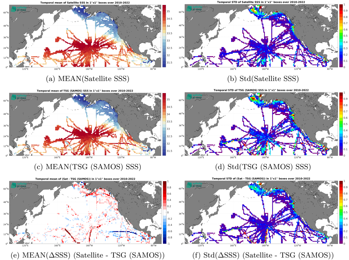
Figure 7: Temporal mean (left) and Std (right) of SSS from CCI SSS L4 Merged-OI v4.41 - 30-day running (ESA) (top), TSG (SAMOS) (middle), and of \Delta SSS (Satellite - TSG (SAMOS)). Only match-up pairs are used to generate these maps.
