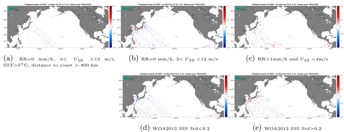
Figure 14: Temporal mean gridded over spatial boxes of size 1^\circ \times 1^\circ of \Delta SSS (CCI SSS L4 Merged-OI v4.41 - 30-day running (ESA) - TSG (LEGOS-DM)) for 5 different subdatasets corresponding to:RR=0 mm/h, 3 < U_{10} < 12 m/s, SST >5^\circ\text{C} , distance to coast > 800 km (a), RR=0 mm/h, 3 < U_{10} < 12 m/s (b), RR >1 mm/h and U_{10} < 4 m/s (c), WOA2013 SSS Std <0.2 (d), WOA2013 SSS Std >0.2 (e).
