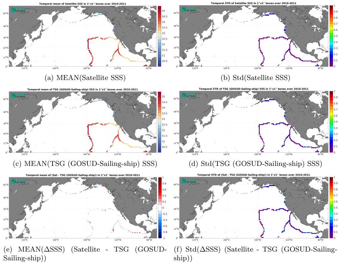
Figure 7: Temporal mean (left) and Std (right) of SSS from CCI SSS L4 Merged-OI v4.41 - 30-day running (ESA) (top), TSG (GOSUD-Sailing-ship) (middle), and of \Delta\text{SSS} (Satellite - TSG (GOSUD-Sailing-ship)). Only match-up pairs are used to generate these maps.
