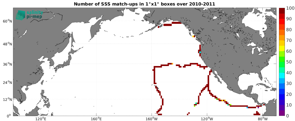
Figure 5: Number of SSS match-ups between TSG (GOSUD-Sailing-ship) SSS and the CCI SSS L4 Merged-OI v4.41 - 30-day running (ESA) SSS product for the North Pacific Ocean Pi-MEP region over 1^\circ \times 1^\circ boxes and for the full satellite product period.
