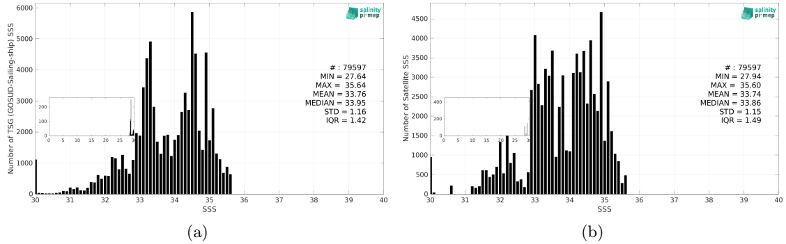
Figure 3: Histograms of SSS from TSG (GOSUD-Sailing-ship) (a) and CCI SSS L4 Merged-OI v4.41 - 30-day running (ESA) (b) considering all match-up pairs per bins of 0.1 over the North Pacific Ocean Pi-MEP region and for the full satellite product period.
