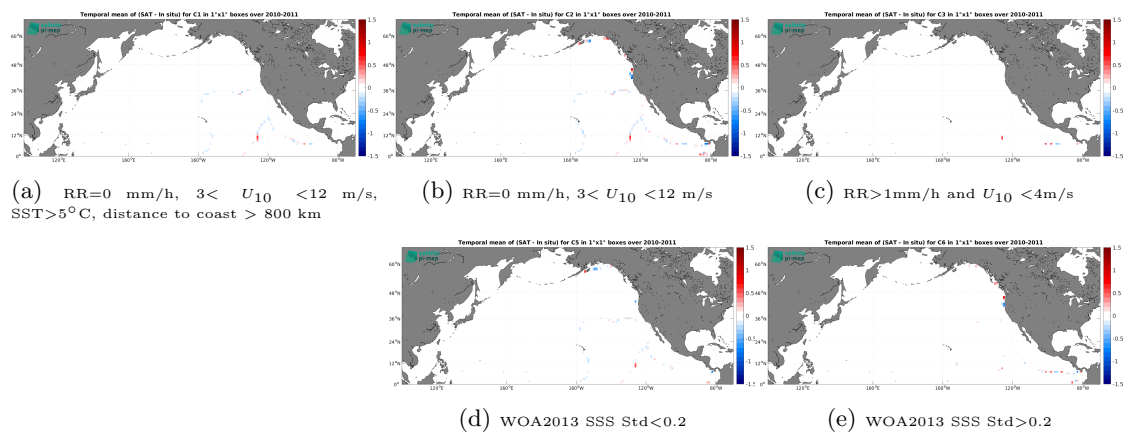
Figure 14: Temporal mean gridded over spatial boxes of size 1^\circ \times 1^\circ of \Delta\text{SSS} (CCI SSS L4 Merged-OI v4.41 - 30-day running (ESA) - TSG (GOSUD-Sailing-ship)) for 5 different subdatasets corresponding to:RR=0 mm/h, 3 < U_{10} < 12 m/s, SST>5°C, distance to coast > 800 km (a), RR=0 mm/h, 3 < U_{10} < 12 m/s (b), RR>1mm/h and U_{10} < 4 m/s (c), WOA2013 SSS Std<0.2 (d), WOA2013 SSS Std>0.2 (e).
