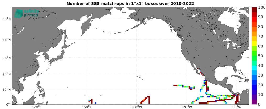
Figure 5: Number of SSS match-ups between TSG (GOSUD-Research-vessel) SSS and the CCI SSS L4 Merged-OI v4.41 - 30-day running (ESA) SSS product for the North Pacific Ocean Pi-MEP region over 1^\circ \times 1^\circ boxes and for the full satellite product period.
