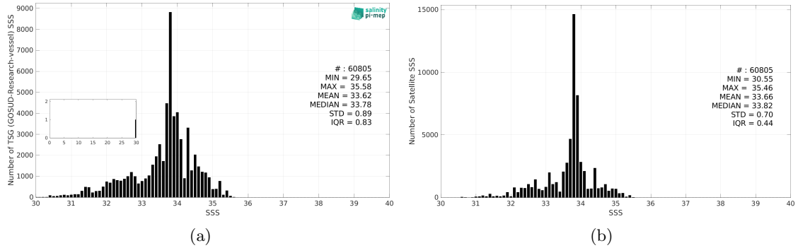
Figure 3: Histograms of SSS from TSG (GOSUD-Research-vessel) (a) and CCI SSS L4 Merged-OI v4.41 - 30-day running (ESA) (b) considering all match-up pairs per bins of 0.1 over the North Pacific Ocean Pi-MEP region and for the full satellite product period.
