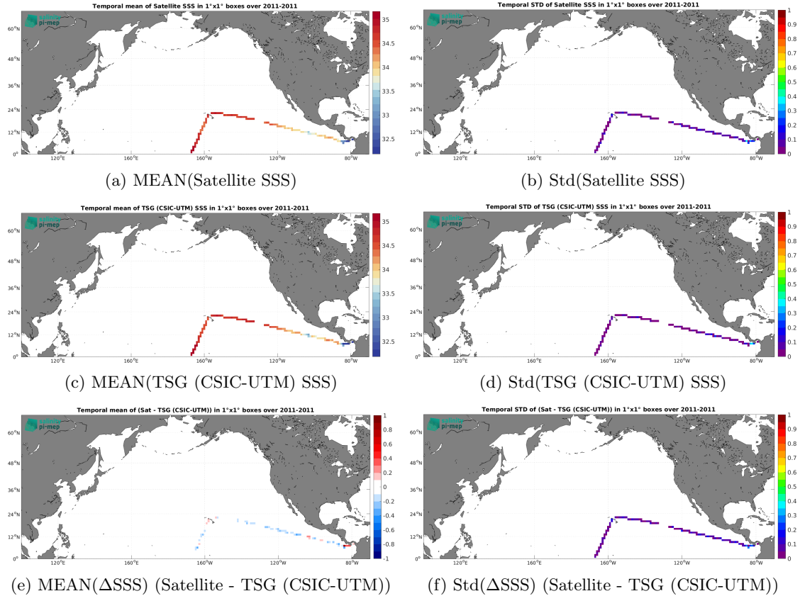
Figure 7: Temporal mean (left) and Std (right) of SSS from CCI SSS L4 Merged-OI v4.41 - 30-day running (ESA) (top), TSG (CSIC-UTM) (middle), and of \Delta\text{SSS} (Satellite - TSG (CSIC-UTM)). Only match-up pairs are used to generate these maps.
