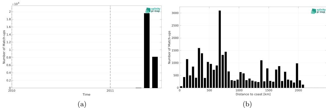
Figure 2: Number of match-ups between TSG (CSIC-UTM) and CCI SSS L4 Merged-OI v4.41 - 30-day running (ESA) SSS as a function of time (a) and as function of the distance to coast (b) over the North Pacific Ocean Pi-MEP region and for the full satellite product period.
