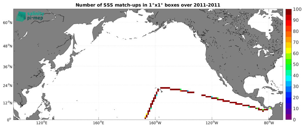
Figure 5: Number of SSS match-ups between TSG (CSIC-UTM) SSS and the CCI SSS L4 Merged-OI v4.41 - 30-day running (ESA) SSS product for the North Pacific Ocean Pi-MEP region over 1^\circ \times 1^\circ boxes and for the full satellite product period.
