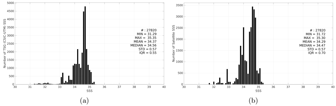
Figure 3: Histograms of SSS from TSG (CSIC-UTM) (a) and CCI SSS L4 Merged-OI v4.41 - 30-day running (ESA) (b) considering all match-up pairs per bins of 0.1 over the North Pacific Ocean Pi-MEP region and for the full satellite product period.
