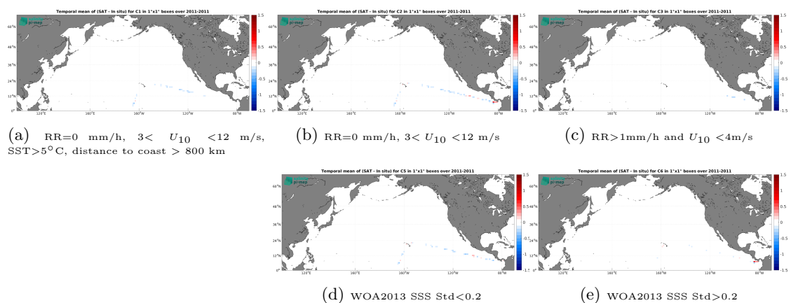
Figure 14: Temporal mean gridded over spatial boxes of size 1^\circ \times 1^\circ of \Delta\text{SSS} (CCI SSS L4 Merged-OI v4.41 - 30-day running (ESA) - TSG (CSIC-UTM)) for 5 different subdatasets corresponding to:RR=0 mm/h, 3 < U_{10} < 12 m/s, SST>5°C, distance to coast > 800 km (a), RR=0 mm/h, 3 < U_{10} < 12 m/s (b), RR>1mm/h and U_{10} < 4 m/s (c), WOA2013 SSS Std<0.2 (d), WOA2013 SSS Std>0.2 (e).
