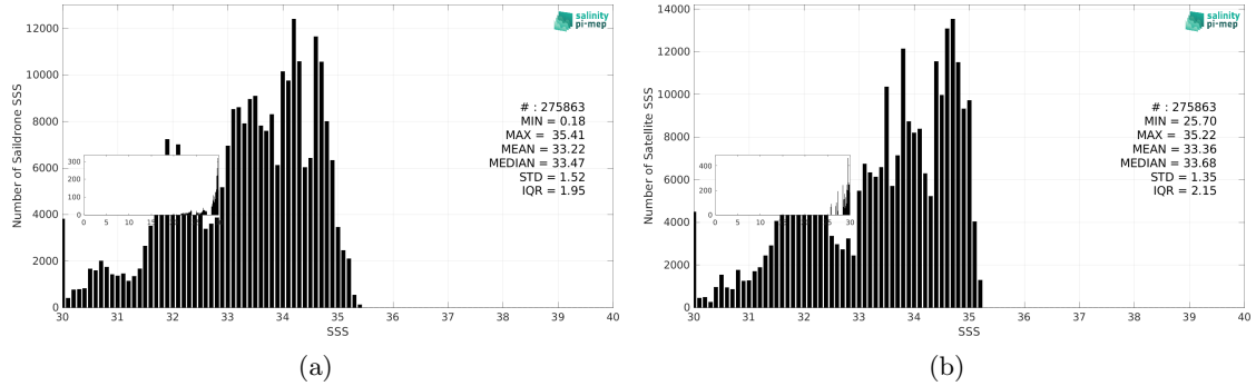
Figure 3: Histograms of SSS from Sailldrone (a) and CCI SSS L4 Merged-OI v4.41 - 30-day running (ESA) (b) considering all match-up pairs per bins of 0.1 over the North Pacific Ocean Pi-MEP region and for the full satellite product period.
