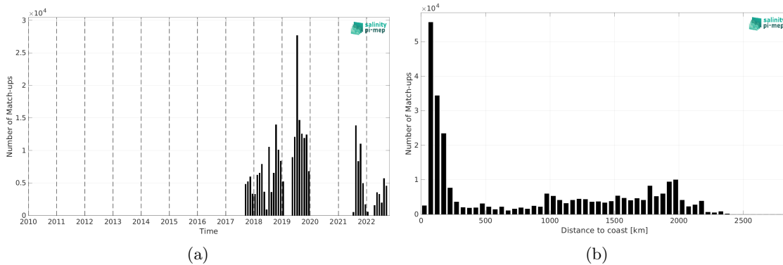
Figure 2: Number of match-ups between Saildrone and CCI SSS L4 Merged-OI v4.41 - 30-day running (ESA) SSS as a function of time (a) and as function of the distance to coast (b) over the North Pacific Ocean Pi-MEP region and for the full satellite product period.
