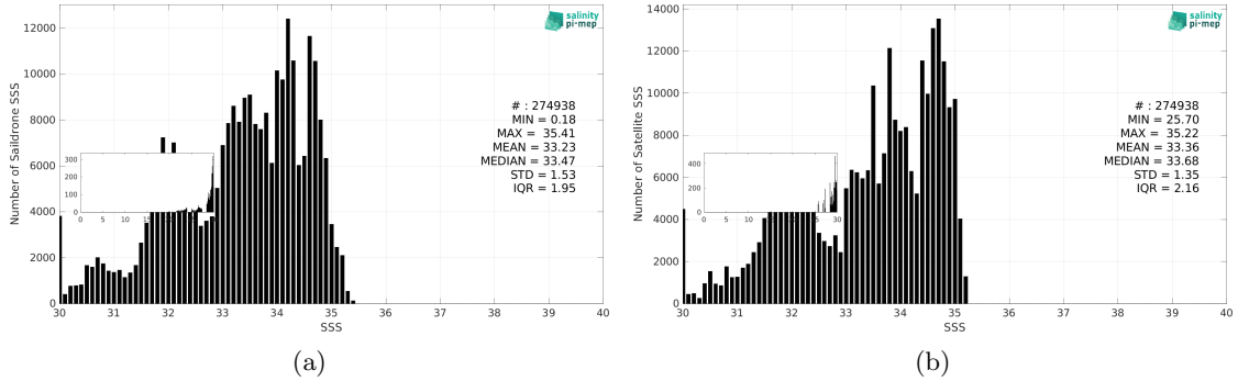
Figure 3: Histograms of SSS from Saildrone (a) and CCI SSS L4 Merged-OI v4.41 - 30-day running (ESA) (b) considering all match-up pairs per bins of 0.1 over the North Pacific Ocean Pi-MEP region and for the full satellite product period.
