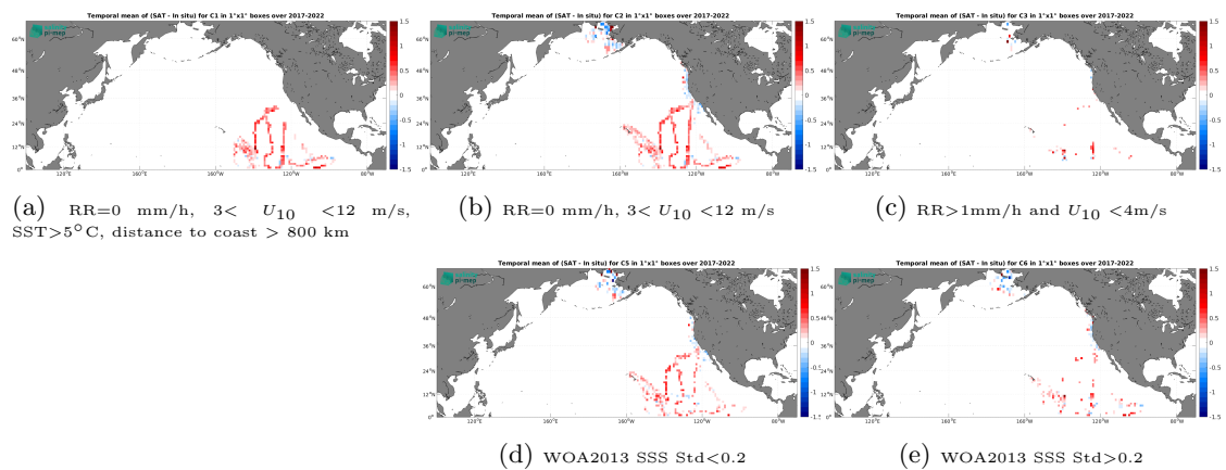
Figure 14: Temporal mean gridded over spatial boxes of size 1^\circ \times 1^\circ of \Delta\text{SSS} (CCI SSS L4 Merged-OI v4.41 - 30-day running (ESA) - Saildrone) for 5 different subdatasets corresponding to:RR=0 mm/h, 3 < U_{10} < 12 m/s, SST>5°C, distance to coast > 800 km (a), RR=0 mm/h, 3 < U_{10} < 12 m/s (b), RR>1mm/h and U_{10} < 4 m/s (c), WOA2013 SSS Std<0.2 (d), WOA2013 SSS Std>0.2 (e).
