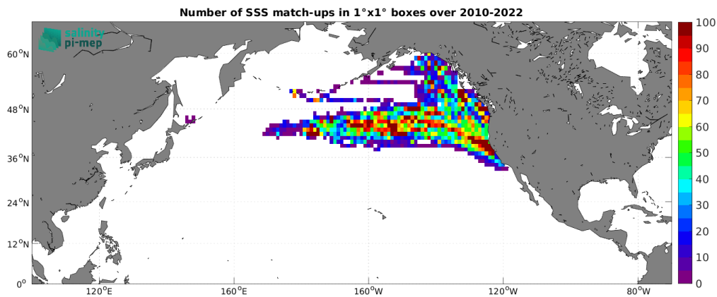
Figure 5: Number of SSS match-ups between Marine mammals SSS and the CCI SSS L4 Merged-OI v4.41 - 30-day running (ESA) SSS product for the North Pacific Ocean Pi-MEP region over 1^\circ \times 1^\circ boxes and for the full satellite product period.
