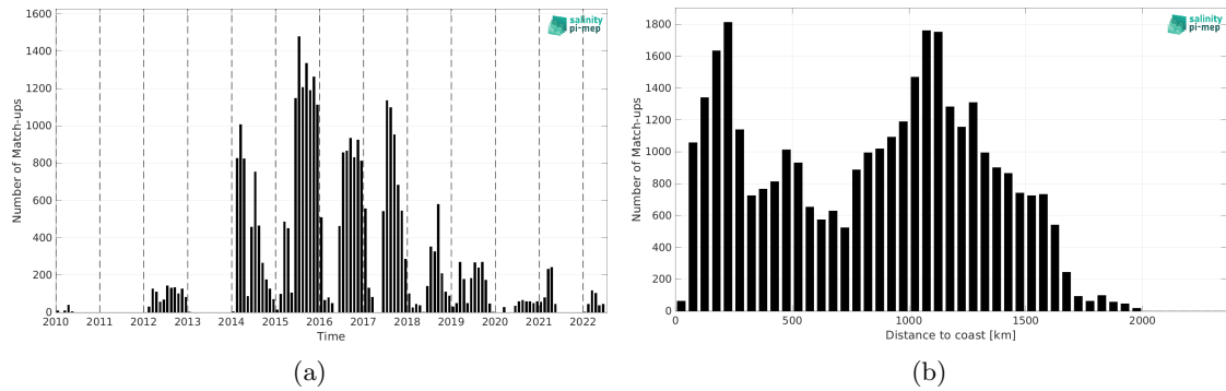
Figure 2: Number of match-ups between Marine mammals and CCI SSS L4 Merged-OI v4.41 - 30-day running (ESA) SSS as a function of time (a) and as function of the distance to coast (b) over the North Pacific Ocean Pi-MEP region and for the full satellite product period.
