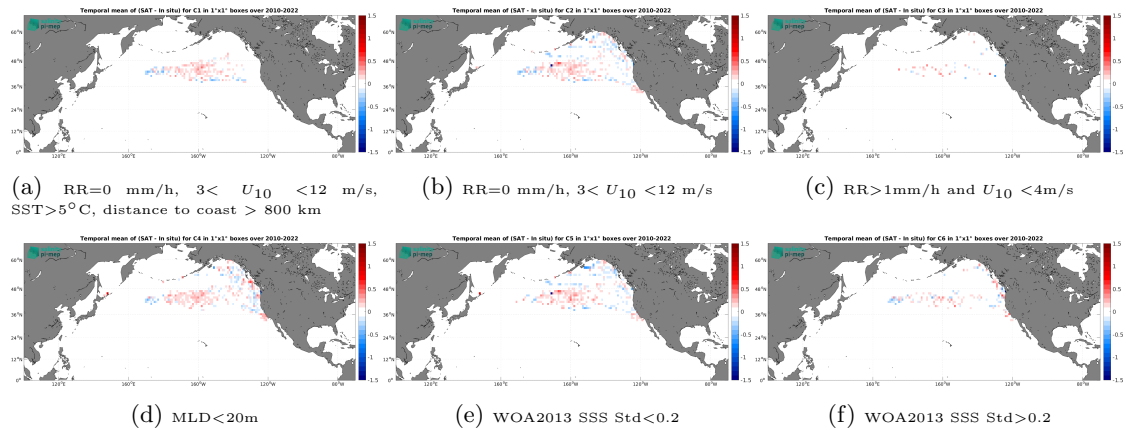
Figure 14: Temporal mean gridded over spatial boxes of size 1^\circ \times 1^\circ of \Delta SSS (CCI SSS L4 Merged-OI v4.41 - 30-day running (ESA) - Marine mammals) for 6 different subdatasets corresponding to:RR=0 mm/h, 3 < U_{10} < 12 m/s, SST >5^\circ C, distance to coast > 800 km (a), RR=0 mm/h, 3 < U_{10} < 12 m/s (b), RR >1 mm/h and U_{10} < 4 m/s (c),MLD <20 m (d),WOA2013 SSS Std <0.2 (e),WOA2013 SSS Std >0.2 (f).
