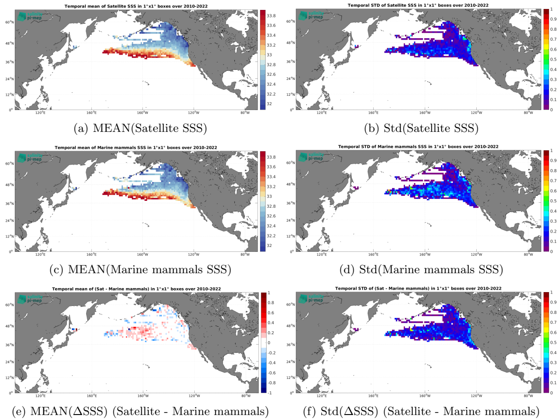
Figure 7: Temporal mean (left) and Std (right) of SSS from CCI SSS L4 Merged-OI v4.41 - 30-day running (ESA) (top), Marine mammals (middle), and of \Delta SSS (Satellite - Marine mammals). Only match-up pairs are used to generate these maps.
