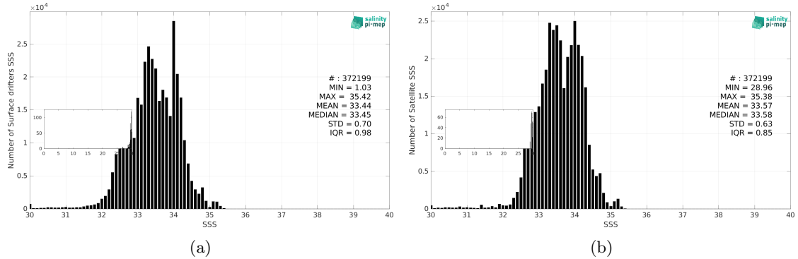
Figure 3: Histograms of SSS from Surface drifters (a) and CCI SSS L4 Merged-OI v4.41 - 30-day running (ESA) (b) considering all match-up pairs per bins of 0.1 over the North Pacific Ocean Pi-MEP region and for the full satellite product period.
