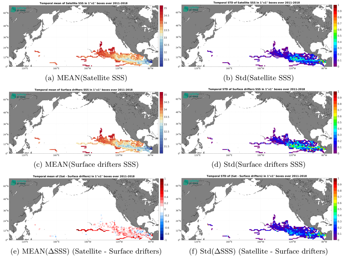
Figure 6: Temporal mean (left) and Std (right) of SSS from CCI SSS L4 Merged-OI v4.41 - 30-day running (ESA) (top), Surface drifters (middle), and of \Delta SSS (Satellite - Surface drifters). Only match-up pairs are used to generate these maps.
