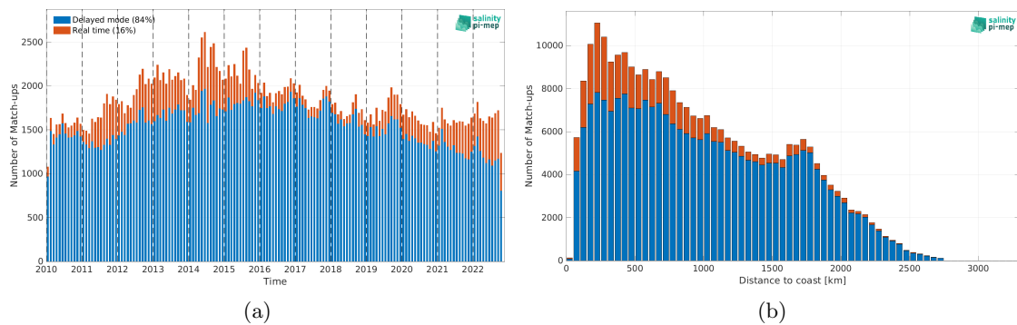
Figure 2: Number of match-ups between Argo and CCI SSS L4 Merged-OI v4.41 - 30-day running (ESA) SSS as a function of time (a) and as function of the distance to coast (b) over the North Pacific Ocean Pi-MEP region and for the full satellite product period.
