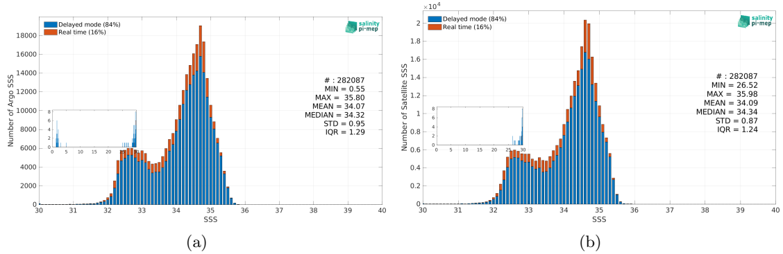
Figure 3: Histograms of SSS from Argo (a) and CCI SSS L4 Merged-OI v4.41 - 30-day running (ESA) (b) considering all match-up pairs per bins of 0.1 over the North Pacific Ocean Pi-MEP region and for the full satellite product period.
