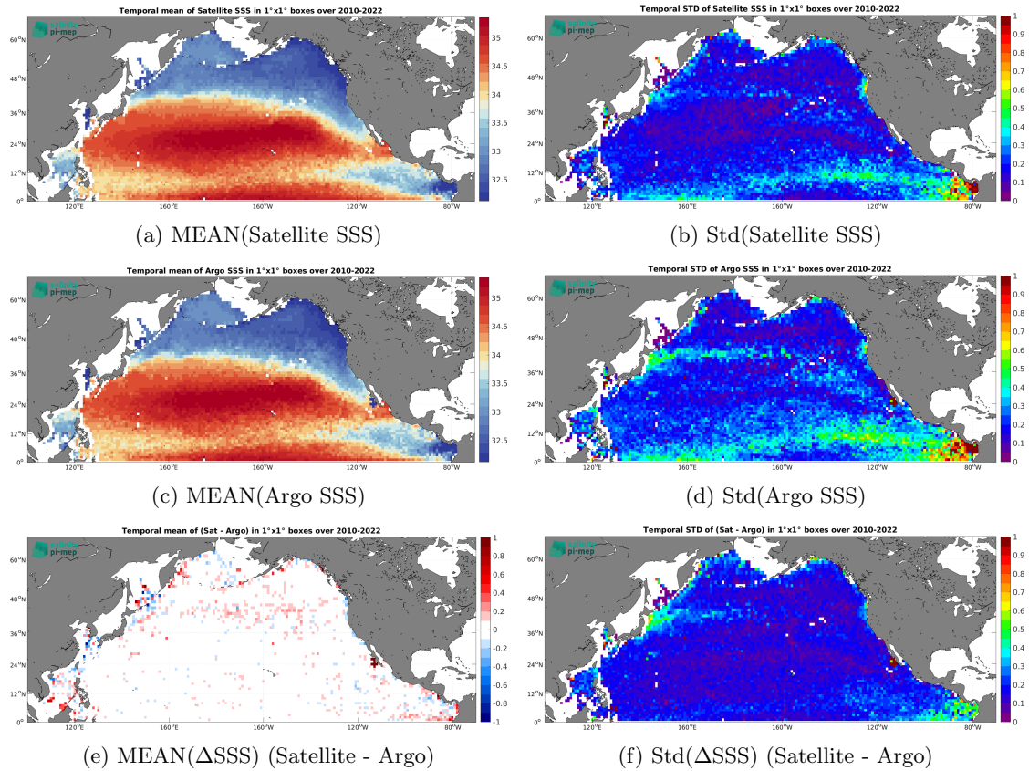
Figure 7: Temporal mean (left) and Std (right) of SSS from CCI SSS L4 Merged-OI v4.41 - 30-day running (ESA) (top), Argo (middle), and of \Delta\text{SSS} (Satellite - Argo). Only match-up pairs are used to generate these maps.
