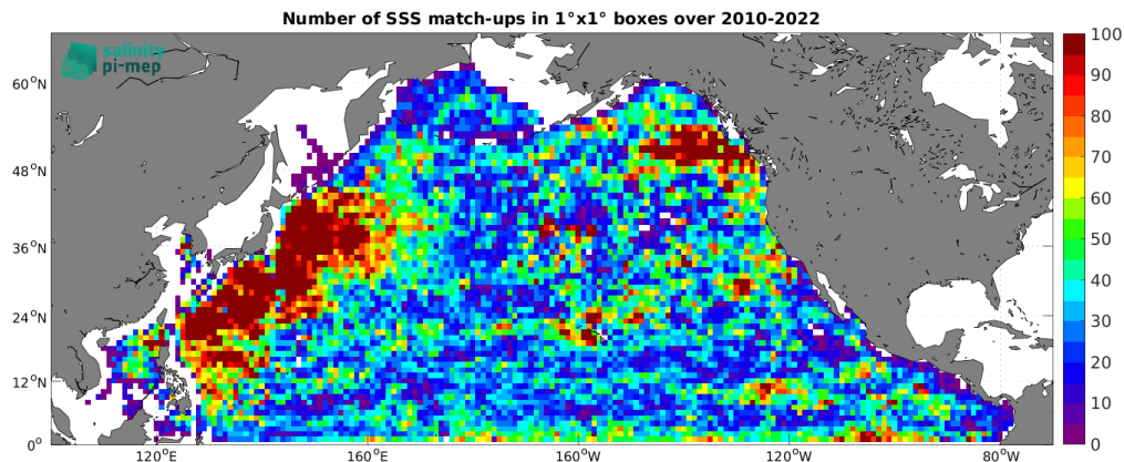
Figure 5: Number of SSS match-ups between Argo SSS and the CCI SSS L4 Merged-OI v4.41 - 30-day running (ESA) SSS product for the North Pacific Ocean Pi-MEP region over 1^\circ \times 1^\circ boxes and for the full satellite product period.
