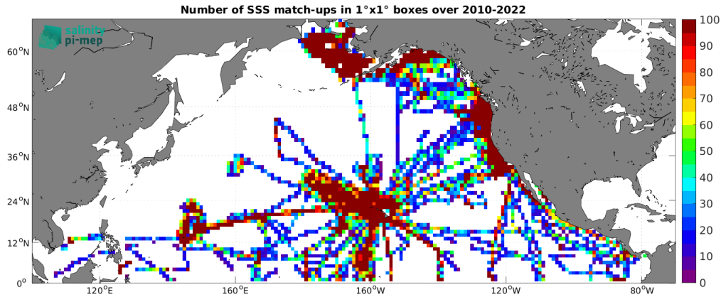
Figure 4: Number of SSS match-ups between TSG (SAMOS) SSS and the CCI SSS L4 Merged-OI v4.4 - 7-day running (ESA) SSS product for the North Pacific Ocean Pi-MEP region over 1^\circ \times 1^\circ boxes and for the full satellite product period.
