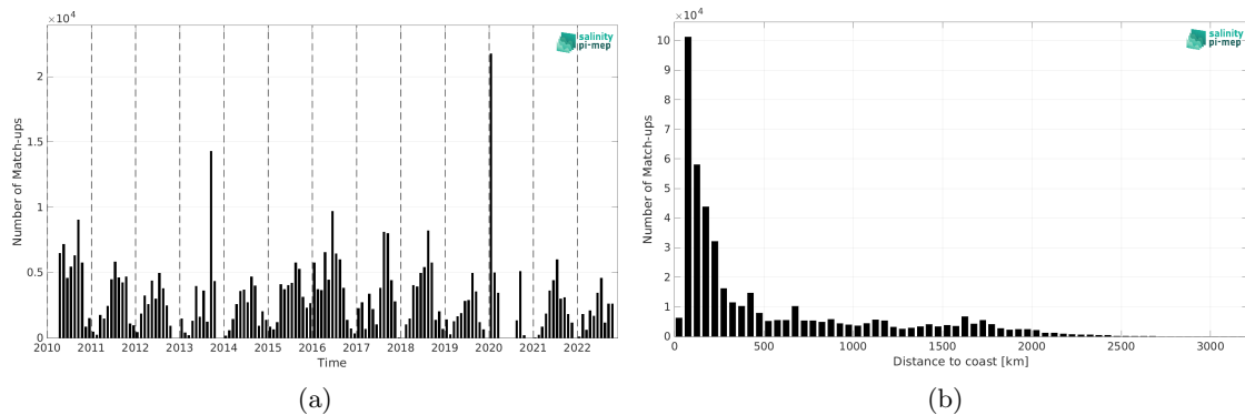
Figure 1: Number of match-ups between TSG (SAMOS) and CCI SSS L4 Merged-OI v4.4 - 7-day running (ESA) SSS as a function of time (a) and as function of the distance to coast (b) over the North Pacific Ocean Pi-MEP region and for the full satellite product period.
