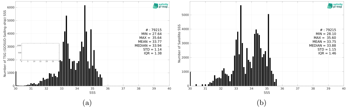
Figure 2: Histograms of SSS from TSG (GOSUD-Sailing-ship) (a) and CCI SSS L4 Merged-OI v4.4 - 7-day running (ESA) (b) considering all match-up pairs per bins of 0.1 over the North Pacific Ocean Pi-MEP region and for the full satellite product period.
