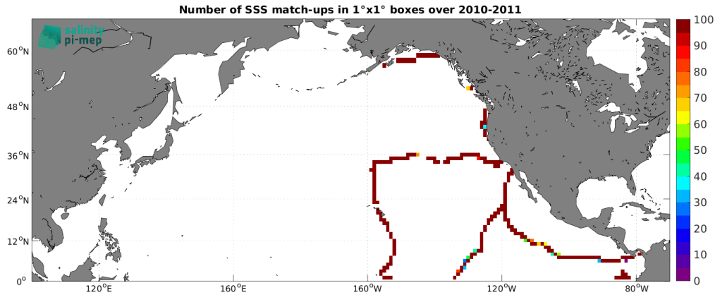
Figure 4: Number of SSS match-ups between TSG (GOSUD-Sailing-ship) SSS and the CCI SSS L4 Merged-OI v4.4 - 7-day running (ESA) SSS product for the North Pacific Ocean Pi-MEP region over 1^\circ \times 1^\circ boxes and for the full satellite product period.
