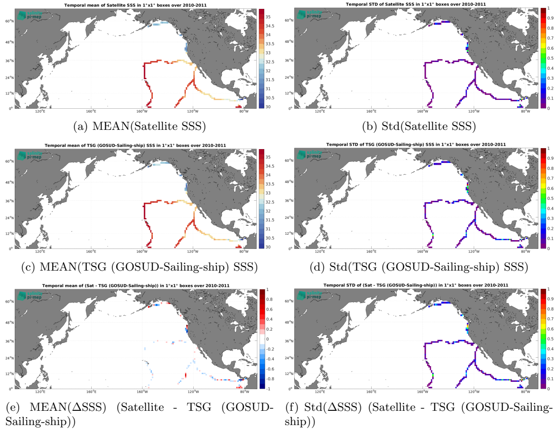
Figure 6: Temporal mean (left) and Std (right) of SSS from CCI SSS L4 Merged-OI v4.4 - 7-day running (ESA) (top), TSG (GOSUD-Sailing-ship) (middle), and of \Delta SSS (Satellite - TSG (GOSUD-Sailing-ship)). Only match-up pairs are used to generate these maps.
