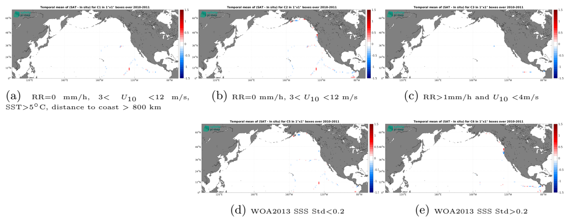
Figure 12: Temporal mean gridded over spatial boxes of size 1^\circ \times 1^\circ of \Delta\text{SSS} (CCI SSS L4 Merged-OI v4.4 - 7-day running (ESA) - TSG (GOSUD-Sailing-ship)) for 5 different subdatasets corresponding to: RR=0 mm/h, 3 < U_{10} < 12 m/s, SST > 5^\circ\text{C} , distance to coast > 800 km (a), RR=0 mm/h, 3 < U_{10} < 12 m/s (b), RR > 1 mm/h and U_{10} < 4 m/s (c), WOA2013 SSS Std < 0.2 (d), WOA2013 SSS Std > 0.2 (e).
