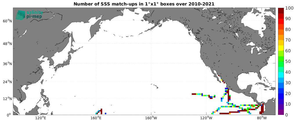
Figure 4: Number of SSS match-ups between TSG (GOSUD-Research-vessel) SSS and the CCI SSS L4 Merged-OI v4.4 - 7-day running (ESA) SSS product for the North Pacific Ocean Pi-MEP region over 1^\circ \times 1^\circ boxes and for the full satellite product period.
