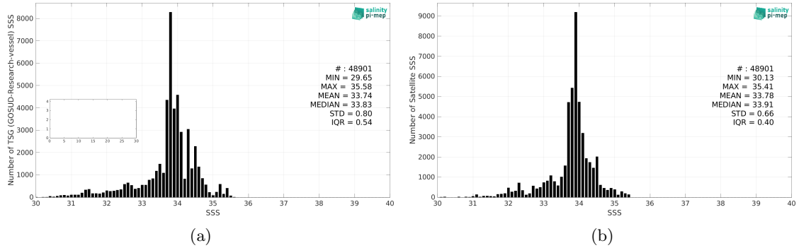
Figure 2: Histograms of SSS from TSG (GOSUD-Research-vessel) (a) and CCI SSS L4 Merged-OI v4.4 - 7-day running (ESA) (b) considering all match-up pairs per bins of 0.1 over the North Pacific Ocean Pi-MEP region and for the full satellite product period.
