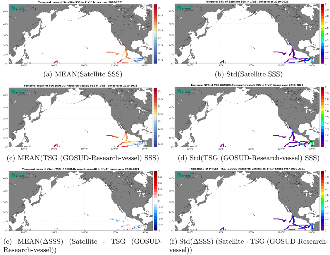
Figure 6: Temporal mean (left) and Std (right) of SSS from CCI SSS L4 Merged-OI v4.4 - 7-day running (ESA) (top), TSG (GOSUD-Research-vessel) (middle), and of \Delta SSS (Satellite - TSG (GOSUD-Research-vessel)). Only match-up pairs are used to generate these maps.
