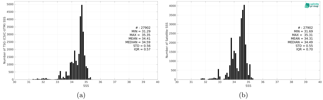
Figure 2: Histograms of SSS from TSG (CSIC-UTM) (a) and CCI SSS L4 Merged-OI v4.4 - 7-day running (ESA) (b) considering all match-up pairs per bins of 0.1 over the North Pacific Ocean Pi-MEP region and for the full satellite product period.
