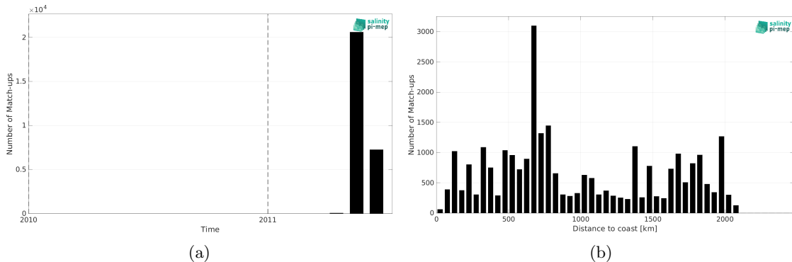
Figure 1: Number of match-ups between TSG (CSIC-UTM) and CCI SSS L4 Merged-OI v4.4 - 7-day running (ESA) SSS as a function of time (a) and as function of the distance to coast (b) over the North Pacific Ocean Pi-MEP region and for the full satellite product period.
