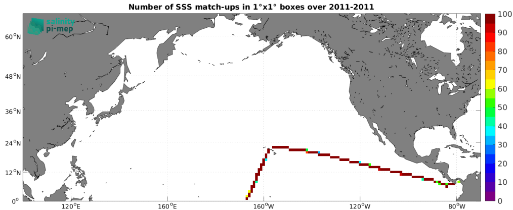
Figure 4: Number of SSS match-ups between TSG (CSIC-UTM) SSS and the CCI SSS L4 Merged-OI v4.4 - 7-day running (ESA) SSS product for the North Pacific Ocean Pi-MEP region over 1^\circ \times 1^\circ boxes and for the full satellite product period.
