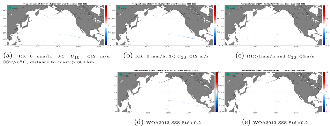
Figure 12: Temporal mean gridded over spatial boxes of size 1^\circ \times 1^\circ of \Delta SSS (CCI SSS L4 Merged-OI v4.4 - 7-day running (ESA) - TSG (CSIC-UTM)) for 5 different subdatasets corresponding to:RR=0 mm/h, 3 < U_{10} < 12 m/s, SST >5^\circ C, distance to coast > 800 km (a), RR=0 mm/h, 3 < U_{10} < 12 m/s (b), RR >1 mm/h and U_{10} < 4 m/s (c), WOA2013 SSS Std <0.2 (d), WOA2013 SSS Std >0.2 (e).
