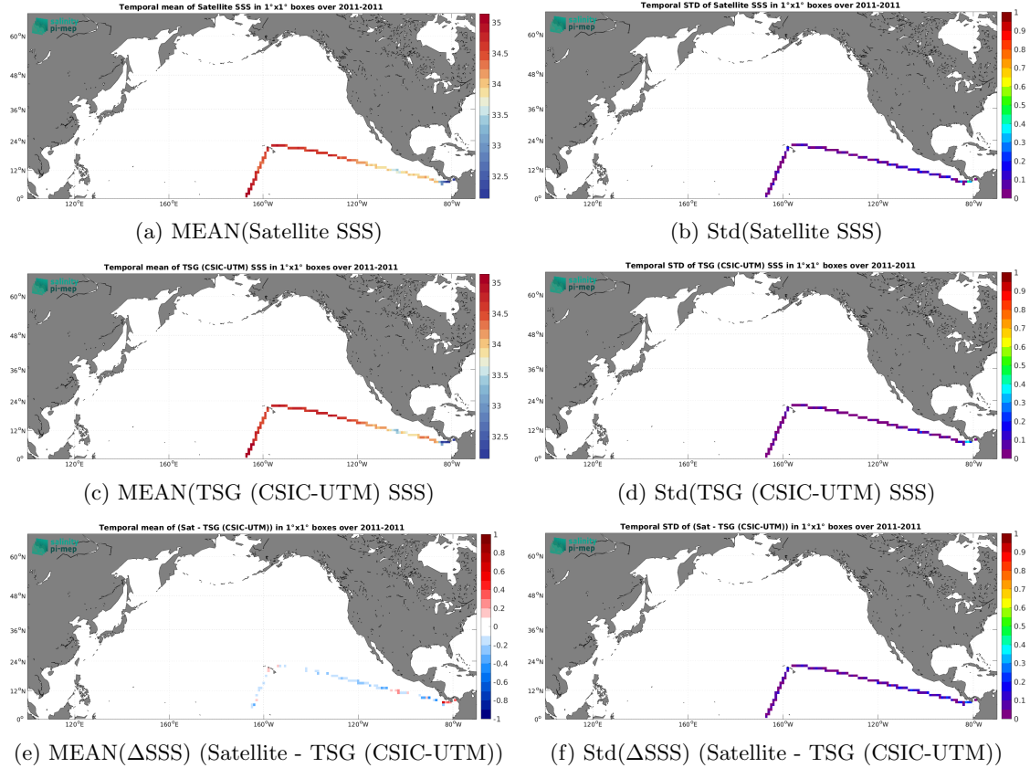
Figure 6: Temporal mean (left) and Std (right) of SSS from CCI SSS L4 Merged-OI v4.4 - 7-day running (ESA) (top), TSG (CSIC-UTM) (middle), and of \Delta SSS (Satellite - TSG (CSIC-UTM)). Only match-up pairs are used to generate these maps.
