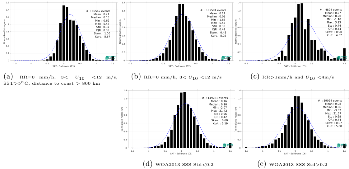
Figure 13: Normalized histogram of \Delta\text{SSS} (CCI SSS L4 Merged-OI v4.4 - 7-day running (ESA) - Sailldrone) for 5 different subdatasets corresponding to: RR=0 mm/h, 3 < U_{10} < 12 m/s, SST>5°C, distance to coast > 800 km (a), RR=0 mm/h, 3 < U_{10} < 12 m/s (b), RR>1mm/h and U_{10} < 4 m/s (c), WOA2013 SSS Std<0.2 (d), WOA2013 SSS Std>0.2 (e).
