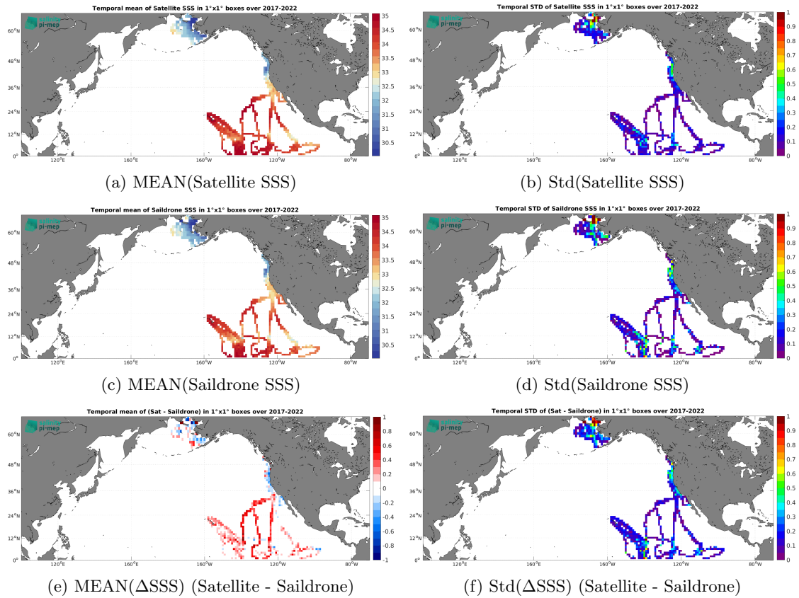
Figure 6: Temporal mean (left) and Std (right) of SSS from CCI SSS L4 Merged-OI v4.4 - 7-day running (ESA) (top), Saildrone (middle), and of \Delta\text{SSS} (Satellite - Saildrone). Only match-up pairs are used to generate these maps.
