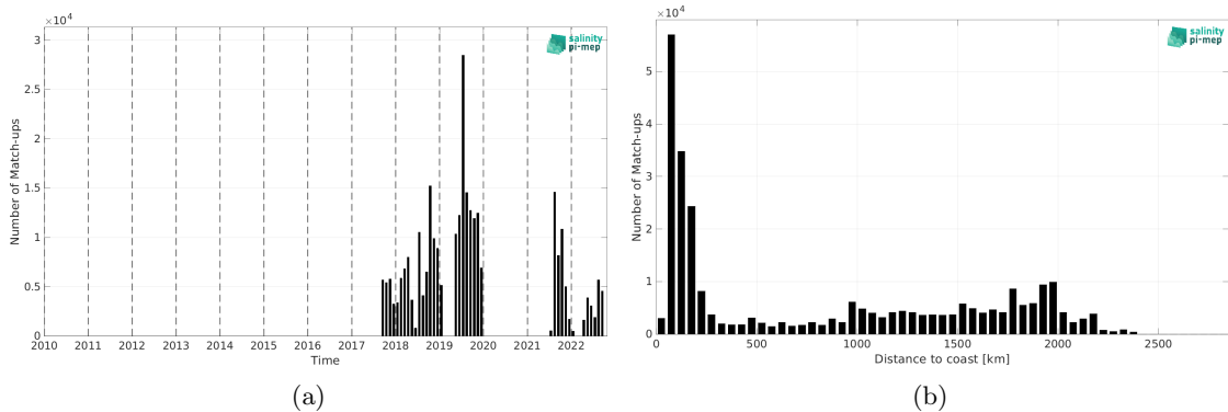
Figure 1: Number of match-ups between Saildrone and CCI SSS L4 Merged-OI v4.4 - 7-day running (ESA) SSS as a function of time (a) and as function of the distance to coast (b) over the North Pacific Ocean Pi-MEP region and for the full satellite product period.
