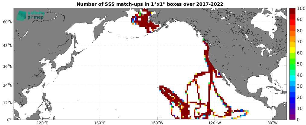
Figure 4: Number of SSS match-ups between Saildrone SSS and the CCI SSS L4 Merged-OI v4.4 - 7-day running (ESA) SSS product for the North Pacific Ocean Pi-MEP region over 1^\circ \times 1^\circ boxes and for the full satellite product period.
