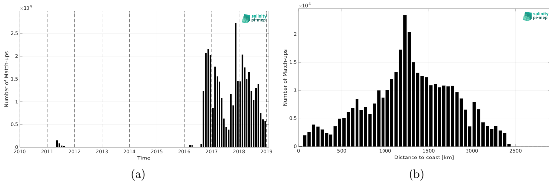
Figure 1: Number of match-ups between Surface drifters and CCI SSS L4 Merged-OI v4.4 - 7-day running (ESA) SSS as a function of time (a) and as function of the distance to coast (b) over the North Pacific Ocean Pi-MEP region and for the full satellite product period.
