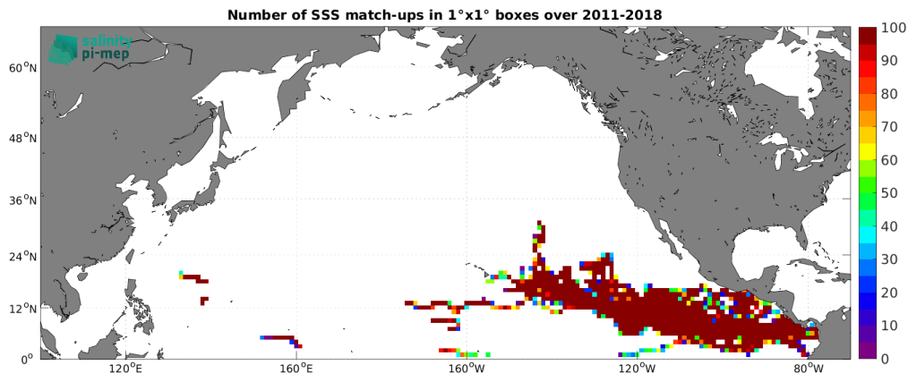
Figure 3: Number of SSS match-ups between Surface drifters SSS and the CCI SSS L4 Merged-OI v4.4 - 7-day running (ESA) SSS product for the North Pacific Ocean Pi-MEP region over 1^\circ \times 1^\circ boxes and for the full satellite product period.
