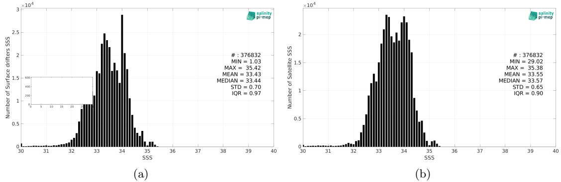
Figure 2: Histograms of SSS from Surface drifters (a) and CCI SSS L4 Merged-OI v4.4 - 7-day running (ESA) (b) considering all match-up pairs per bins of 0.1 over the North Pacific Ocean Pi-MEP region and for the full satellite product period.
