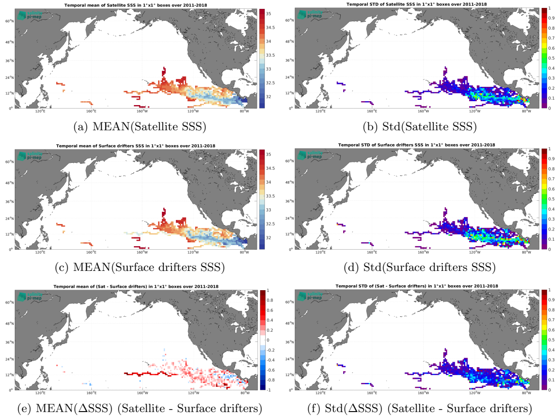
Figure 5: Temporal mean (left) and Std (right) of SSS from CCI SSS L4 Merged-OI v4.4 - 7-day running (ESA) (top), Surface drifters (middle), and of \Delta SSS (Satellite - Surface drifters). Only match-up pairs are used to generate these maps.
