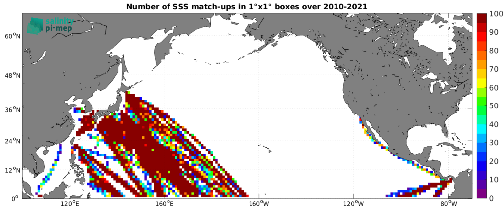
Figure 4: Number of SSS match-ups between TSG (LEGOS-DM) SSS and the CCI SSS L4 Merged-OI v4.4 - 30-day running (ESA) SSS product for the North Pacific Ocean Pi-MEP region over 1^\circ \times 1^\circ boxes and for the full satellite product period.
