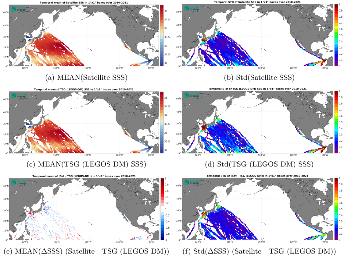
Figure 6: Temporal mean (left) and Std (right) of SSS from CCI SSS L4 Merged-OI v4.4 - 30-day running (ESA) (top), TSG (LEGOS-DM) (middle), and of \Delta\text{SSS} (Satellite - TSG (LEGOS-DM)). Only match-up pairs are used to generate these maps.
