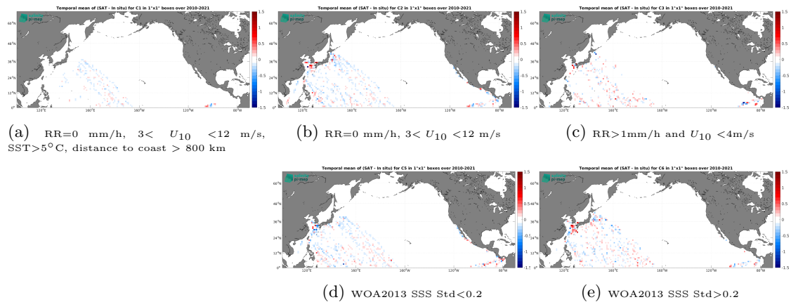
Figure 12: Temporal mean gridded over spatial boxes of size 1^\circ \times 1^\circ of \Delta SSS (CCI SSS L4 Merged-OI v4.4 - 30-day running (ESA) - TSG (LEGOS-DM)) for 5 different subdatasets corresponding to:RR=0 mm/h, 3 < U_{10} < 12 m/s, SST >5^\circ C, distance to coast > 800 km (a), RR=0 mm/h, 3 < U_{10} < 12 m/s (b), RR >1 mm/h and U_{10} < 4 m/s (c), WOA2013 SSS Std <0.2 (d), WOA2013 SSS Std >0.2 (e).
