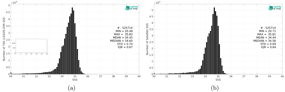
Figure 2: Histograms of SSS from TSG (LEGOS-DM) (a) and CCI SSS L4 Merged-OI v4.4 - 30-day running (ESA) (b) considering all match-up pairs per bins of 0.1 over the North Pacific Ocean Pi-MEP region and for the full satellite product period.
