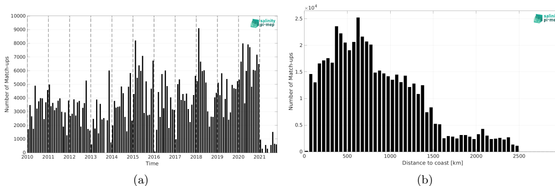
Figure 1: Number of match-ups between TSG (LEGOS-DM) and CCI SSS L4 Merged-OI v4.4 - 30-day running (ESA) SSS as a function of time (a) and as function of the distance to coast (b) over the North Pacific Ocean Pi-MEP region and for the full satellite product period.
