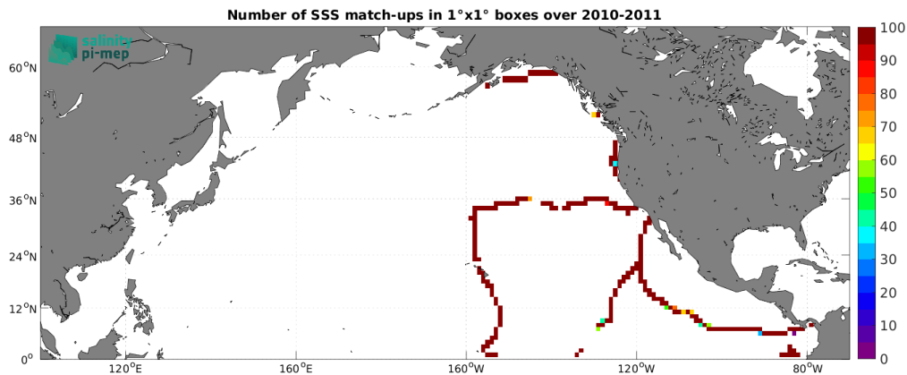
Figure 4: Number of SSS match-ups between TSG (GOSUD-Sailing-ship) SSS and the CCI SSS L4 Merged-OI v4.4 - 30-day running (ESA) SSS product for the North Pacific Ocean Pi-MEP region over 1^\circ \times 1^\circ boxes and for the full satellite product period.
