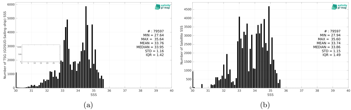
Figure 2: Histograms of SSS from TSG (GOSUD-Sailing-ship) (a) and CCI SSS L4 Merged-OI v4.4 - 30-day running (ESA) (b) considering all match-up pairs per bins of 0.1 over the North Pacific Ocean Pi-MEP region and for the full satellite product period.
