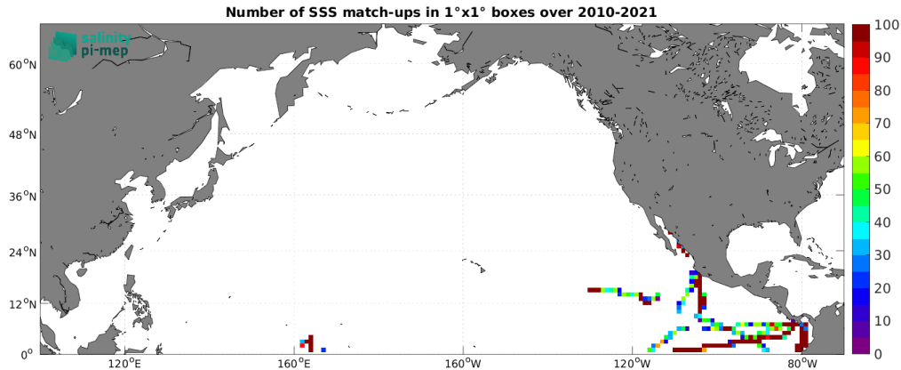
Figure 4: Number of SSS match-ups between TSG (GOSUD-Research-vessel) SSS and the CCI SSS L4 Merged-OI v4.4 - 30-day running (ESA) SSS product for the North Pacific Ocean Pi-MEP region over 1^\circ \times 1^\circ boxes and for the full satellite product period.
