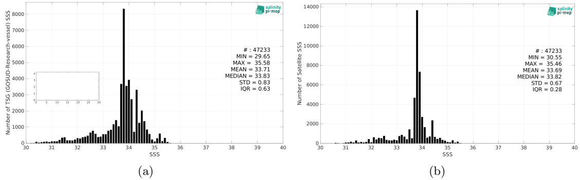
Figure 2: Histograms of SSS from TSG (GOSUD-Research-vessel) (a) and CCI SSS L4 Merged-OI v4.4 - 30-day running (ESA) (b) considering all match-up pairs per bins of 0.1 over the North Pacific Ocean Pi-MEP region and for the full satellite product period.
