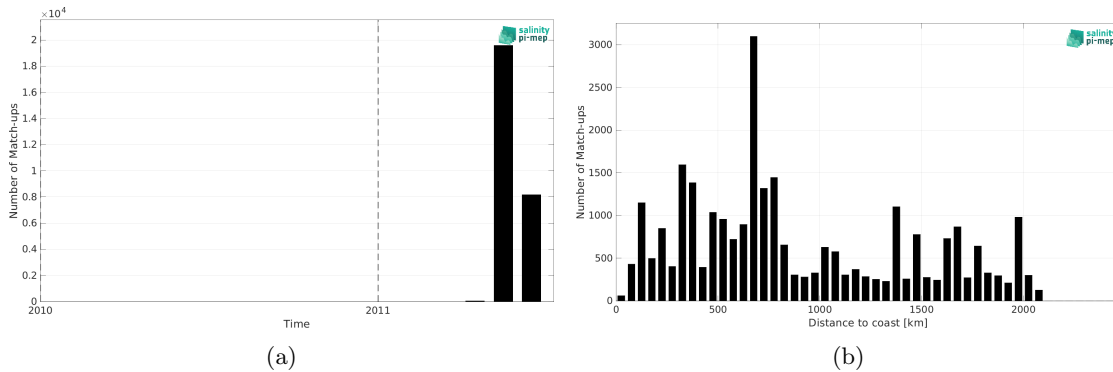
Figure 1: Number of match-ups between TSG (CSIC-UTM) and CCI SSS L4 Merged-OI v4.4 - 30-day running (ESA) SSS as a function of time (a) and as function of the distance to coast (b) over the North Pacific Ocean Pi-MEP region and for the full satellite product period.
