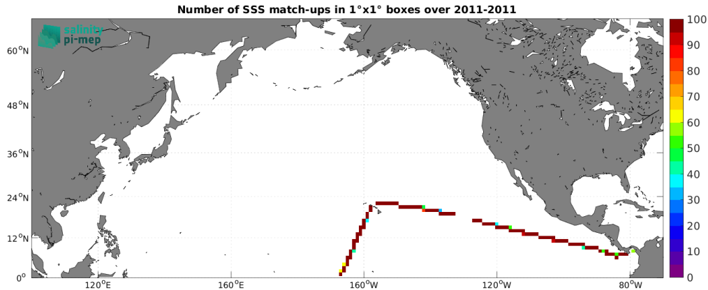
Figure 4: Number of SSS match-ups between TSG (CSIC-UTM) SSS and the CCI SSS L4 Merged-OI v4.4 - 30-day running (ESA) SSS product for the North Pacific Ocean Pi-MEP region over 1^\circ \times 1^\circ boxes and for the full satellite product period.
