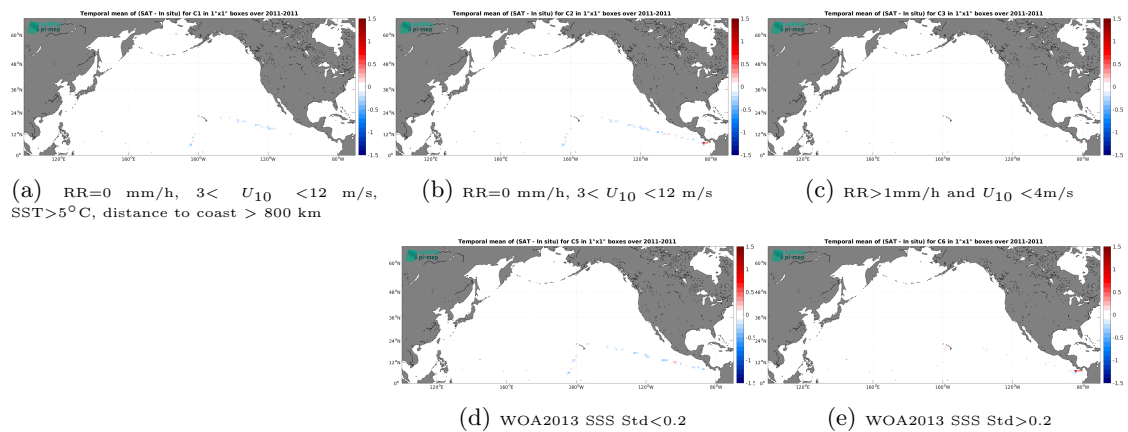
Figure 12: Temporal mean gridded over spatial boxes of size 1^\circ \times 1^\circ of \Delta SSS (CCI SSS L4 Merged-OI v4.4 - 30-day running (ESA) - TSG (CSIC-UTM)) for 5 different subdatasets corresponding to: RR=0 mm/h, 3 < U_{10} < 12 m/s, SST > 5^\circ C , distance to coast > 800 km (a), RR=0 mm/h, 3 < U_{10} < 12 m/s (b), RR > 1 mm/h and U_{10} < 4 m/s (c), WOA2013 SSS Std < 0.2 (d), WOA2013 SSS Std > 0.2 (e).
