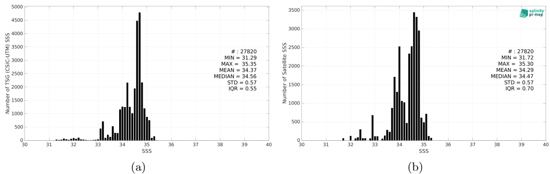
Figure 2: Histograms of SSS from TSG (CSIC-UTM) (a) and CCI SSS L4 Merged-OI v4.4 - 30-day running (ESA) (b) considering all match-up pairs per bins of 0.1 over the North Pacific Ocean Pi-MEP region and for the full satellite product period.
