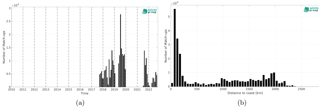
Figure 1: Number of match-ups between Saildrone and CCI SSS L4 Merged-OI v4.4 - 30-day running (ESA) SSS as a function of time (a) and as function of the distance to coast (b) over the North Pacific Ocean Pi-MEP region and for the full satellite product period.
