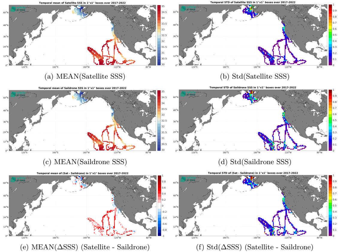
Figure 6: Temporal mean (left) and Std (right) of SSS from CCI SSS L4 Merged-OI v4.4 - 30-day running (ESA) (top), Saildrone (middle), and of \Delta\text{SSS} (Satellite - Saildrone). Only match-up pairs are used to generate these maps.
