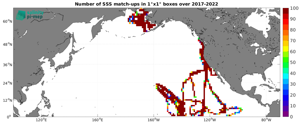
Figure 4: Number of SSS match-ups between Saildrone SSS and the CCI SSS L4 Merged-OI v4.4 - 30-day running (ESA) SSS product for the North Pacific Ocean Pi-MEP region over 1^\circ \times 1^\circ boxes and for the full satellite product period.
