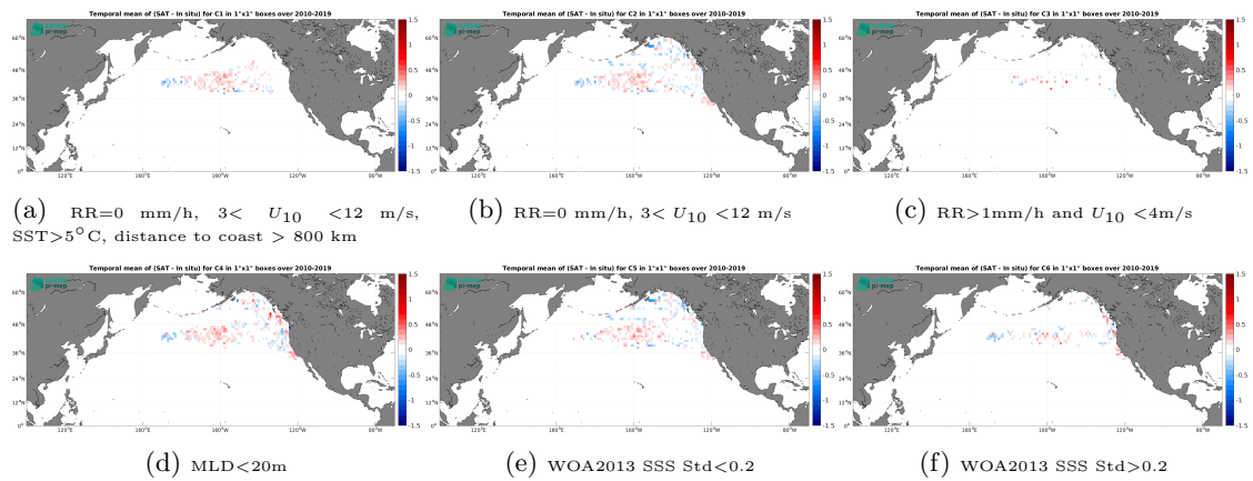
Figure 12: Temporal mean gridded over spatial boxes of size 1^\circ \times 1^\circ of \Delta SSS (CCI SSS L4 Merged-OI v4.4 - 30-day running (ESA) - Marine mammals) for 6 different subdatasets corresponding to:RR=0 mm/h, 3 < U_{10} < 12 m/s, SST >5^\circ C, distance to coast > 800 km (a), RR=0 mm/h, 3 < U_{10} < 12 m/s (b), RR >1 mm/h and U_{10} < 4 m/s (c),MLD <20 m (d),WOA2013 SSS Std <0.2 (e),WOA2013 SSS Std >0.2 (f).
