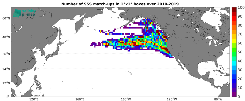
Figure 4: Number of SSS match-ups between Marine mammals SSS and the CCI SSS L4 Merged-OI v4.4 - 30-day running (ESA) SSS product for the North Pacific Ocean Pi-MEP region over 1^\circ \times 1^\circ boxes and for the full satellite product period.
