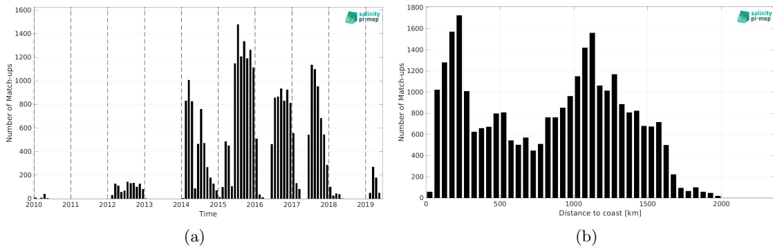
Figure 1: Number of match-ups between Marine mammals and CCI SSS L4 Merged-OI v4.4 - 30-day running (ESA) SSS as a function of time (a) and as function of the distance to coast (b) over the North Pacific Ocean Pi-MEP region and for the full satellite product period.
