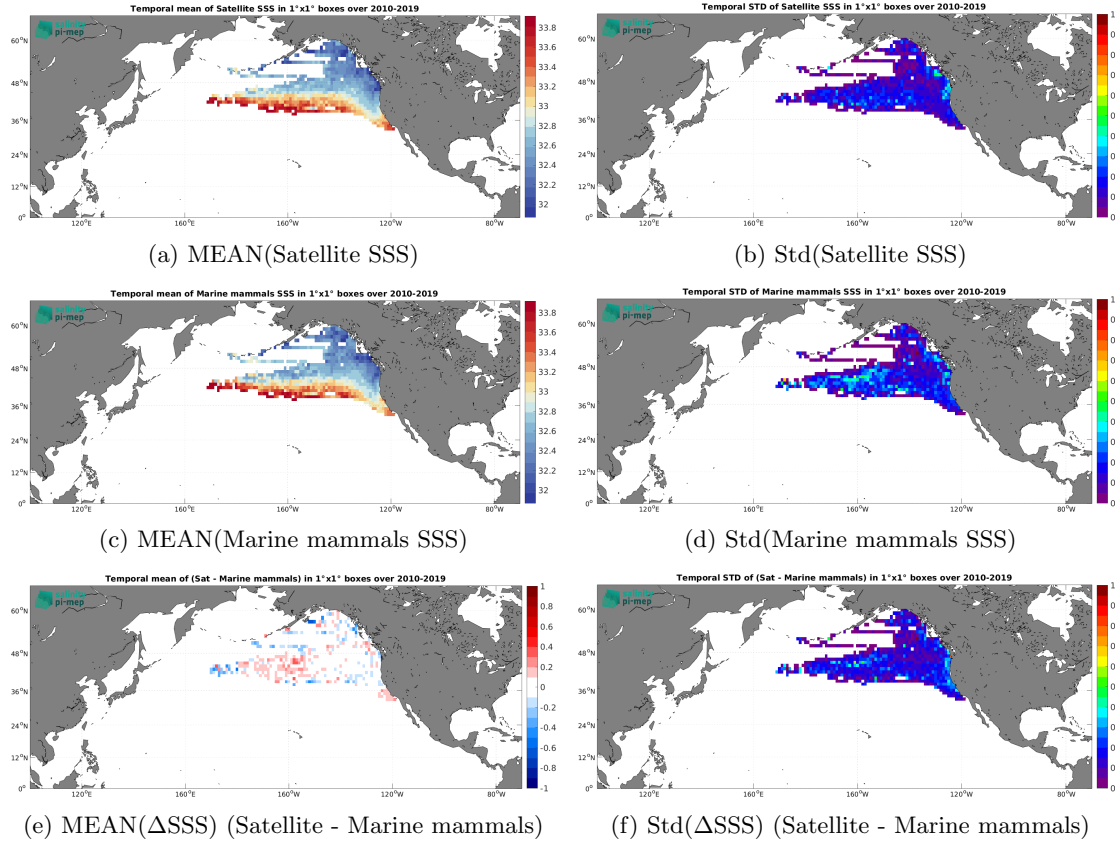
Figure 6: Temporal mean (left) and Std (right) of SSS from CCI SSS L4 Merged-OI v4.4 - 30-day running (ESA) (top), Marine mammals (middle), and of \Delta SSS (Satellite - Marine mammals). Only match-up pairs are used to generate these maps.
