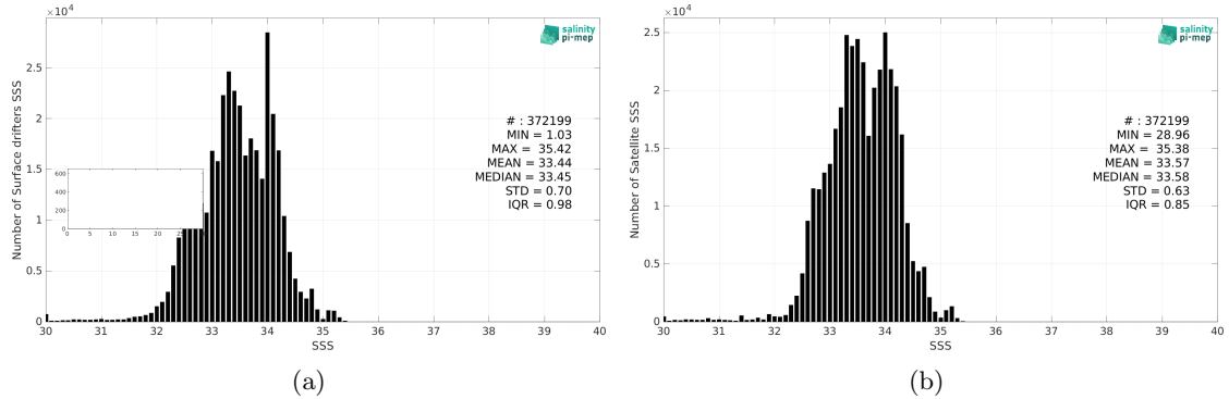
Figure 2: Histograms of SSS from Surface drifters (a) and CCI SSS L4 Merged-OI v4.4 - 30-day running (ESA) (b) considering all match-up pairs per bins of 0.1 over the North Pacific Ocean Pi-MEP region and for the full satellite product period.
