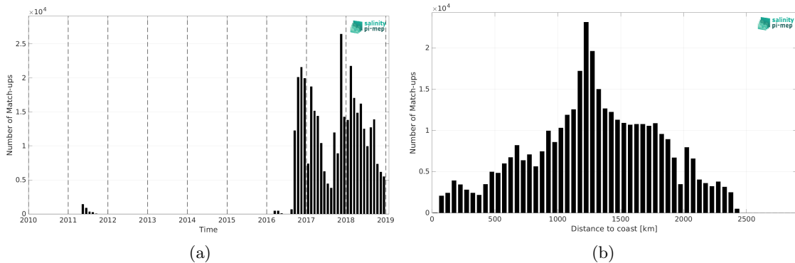
Figure 1: Number of match-ups between Surface drifters and CCI SSS L4 Merged-OI v4.4 - 30-day running (ESA) SSS as a function of time (a) and as function of the distance to coast (b) over the North Pacific Ocean Pi-MEP region and for the full satellite product period.
