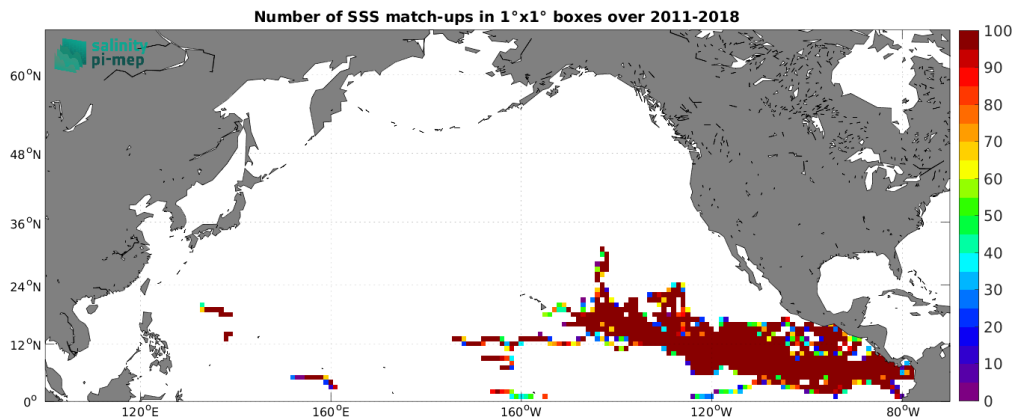
Figure 3: Number of SSS match-ups between Surface drifters SSS and the CCI SSS L4 Merged-OI v4.4 - 30-day running (ESA) SSS product for the North Pacific Ocean Pi-MEP region over 1^\circ \times 1^\circ boxes and for the full satellite product period.
