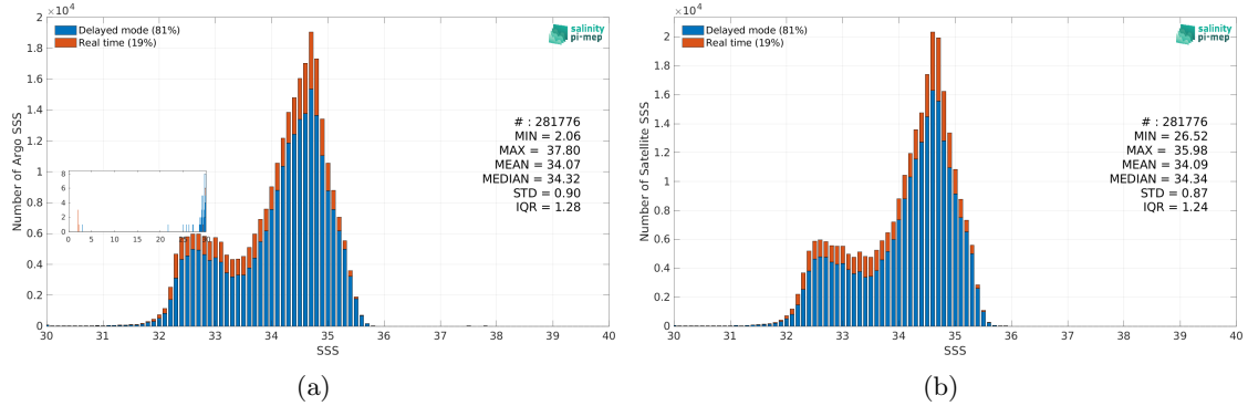
Figure 2: Histograms of SSS from Argo (a) and CCI SSS L4 Merged-OI v4.4 - 30-day running (ESA) (b) considering all match-up pairs per bins of 0.1 over the North Pacific Ocean Pi-MEP region and for the full satellite product period.
