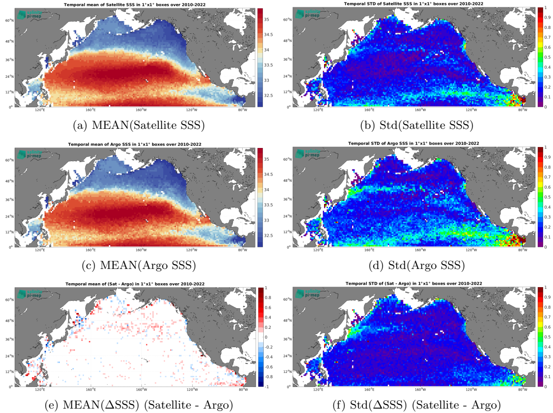
Figure 6: Temporal mean (left) and Std (right) of SSS from CCI SSS L4 Merged-OI v4.4 - 30-day running (ESA) (top), Argo (middle), and of \Delta\text{SSS} (Satellite - Argo). Only match-up pairs are used to generate these maps.
