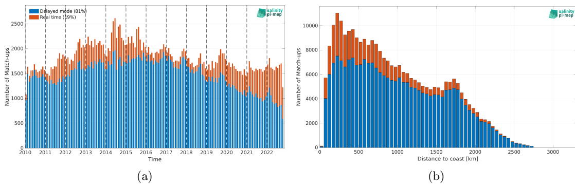
Figure 1: Number of match-ups between Argo and CCI SSS L4 Merged-OI v4.4 - 30-day running (ESA) SSS as a function of time (a) and as function of the distance to coast (b) over the North Pacific Ocean Pi-MEP region and for the full satellite product period.
