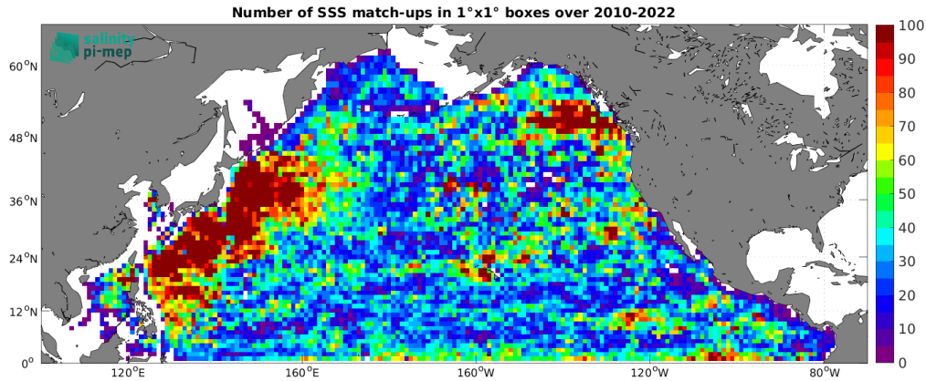
Figure 4: Number of SSS match-ups between Argo SSS and the CCI SSS L4 Merged-OI v4.4 - 30-day running (ESA) SSS product for the North Pacific Ocean Pi-MEP region over 1^\circ \times 1^\circ boxes and for the full satellite product period.
