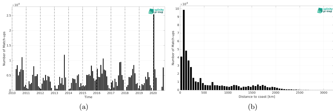
Figure 1: Number of match-ups between TSG (SAMOS) and CCI SSS L4 Merged-OI v3.2 - 7-day running (ESA) SSS as a function of time (a) and as function of the distance to coast (b) over the North Pacific Ocean Pi-MEP region and for the full satellite product period.
