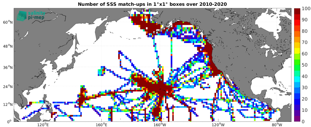
Figure 4: Number of SSS match-ups between TSG (SAMOS) SSS and the CCI SSS L4 Merged-OI v3.2 - 7-day running (ESA) SSS product for the North Pacific Ocean Pi-MEP region over 1^\circ \times 1^\circ boxes and for the full satellite product period.
