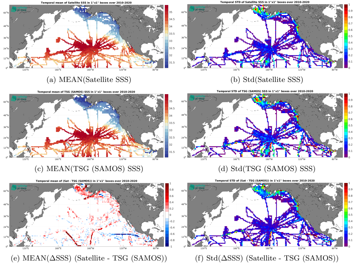
Figure 6: Temporal mean (left) and Std (right) of SSS from CCI SSS L4 Merged-OI v3.2 - 7-day running (ESA) (top), TSG (SAMOS) (middle), and of \Delta\text{SSS} (Satellite - TSG (SAMOS)). Only match-up pairs are used to generate these maps.
