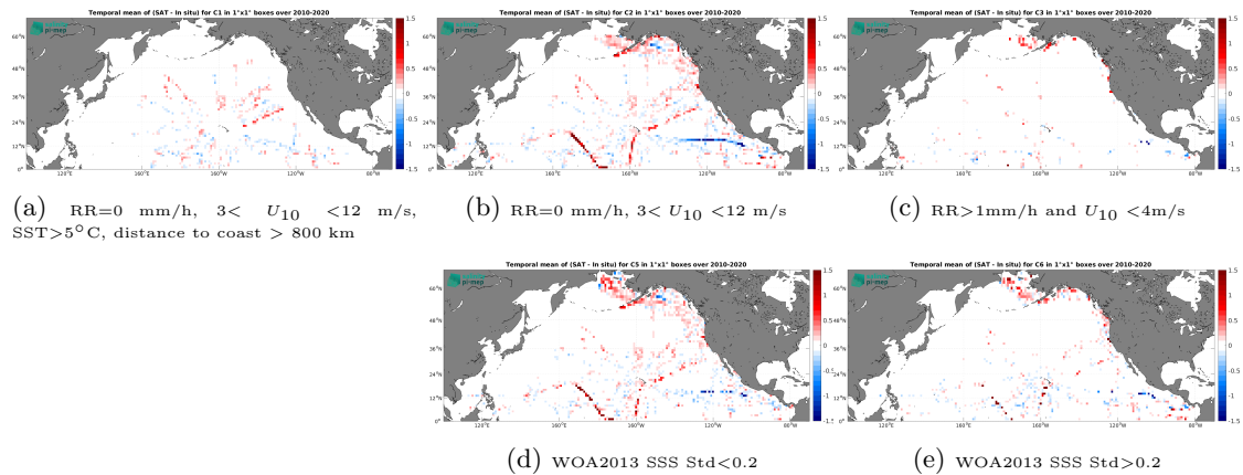
Figure 12: Temporal mean gridded over spatial boxes of size 1^\circ \times 1^\circ of \Delta\text{SSS} (CCI SSS L4 Merged-OI v3.2 - 7-day running (ESA) - TSG (SAMOS)) for 5 different subdatasets corresponding to:RR=0 mm/h, 3 < U_{10} < 12 m/s, SST >5^\circ\text{C} , distance to coast > 800 km (a), RR=0 mm/h, 3 < U_{10} < 12 m/s (b), RR >1 mm/h and U_{10} < 4 m/s (c), WOA2013 SSS Std <0.2 (d), WOA2013 SSS Std >0.2 (e).
