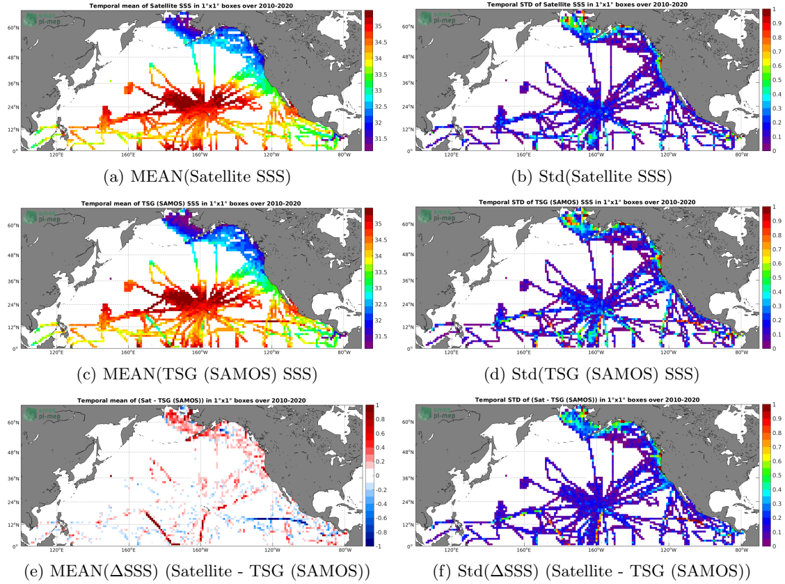
Figure 6: Temporal mean (left) and Std (right) of SSS from CCI SSS L4 Merged-OI v3.2 - 7-day running (ESA) (top), TSG (SAMOS) (middle), and of \Delta SSS (Satellite - TSG (SAMOS)). Only match-up pairs are used to generate these maps.
