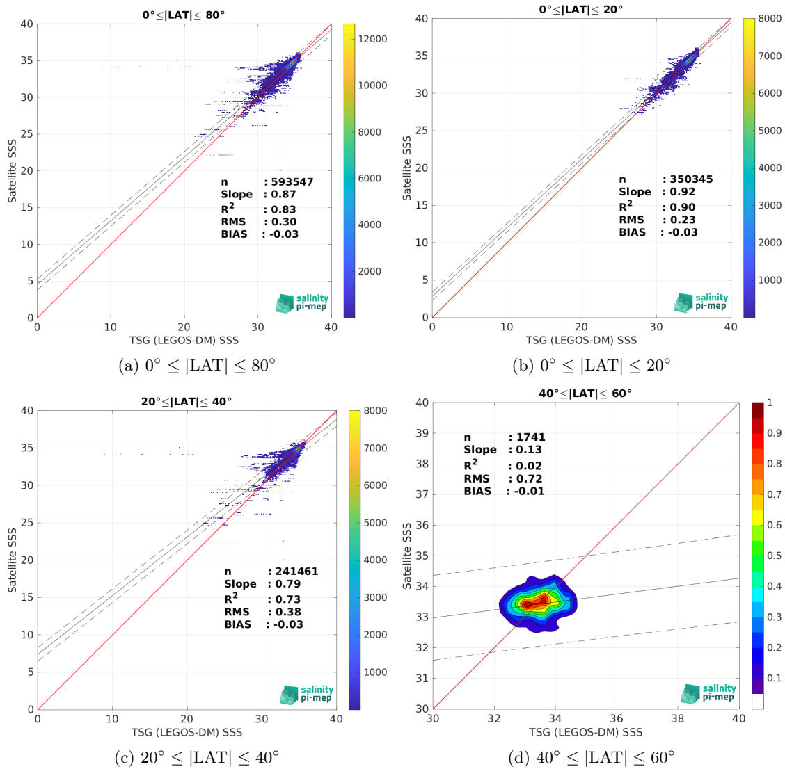
Figure 9: Contour maps of the concentration of CCI SSS L4 Merged-OI v3.2 - 7-day running (ESA) SSS (y-axis) versus TSG (LEGOS-DM) SSS (x-axis) at match-up pairs for different latitude bands. For each plot, the red line shows x=y . The black thin and dashed lines indicate a linear fit through the data cloud and the \pm 95\% confidence levels, respectively. The number match-up pairs n , the slope and R^2 coefficient of the linear fit, the root mean square (RMS) and the mean bias between satellite and in situ data are indicated for each latitude band in each plots.
