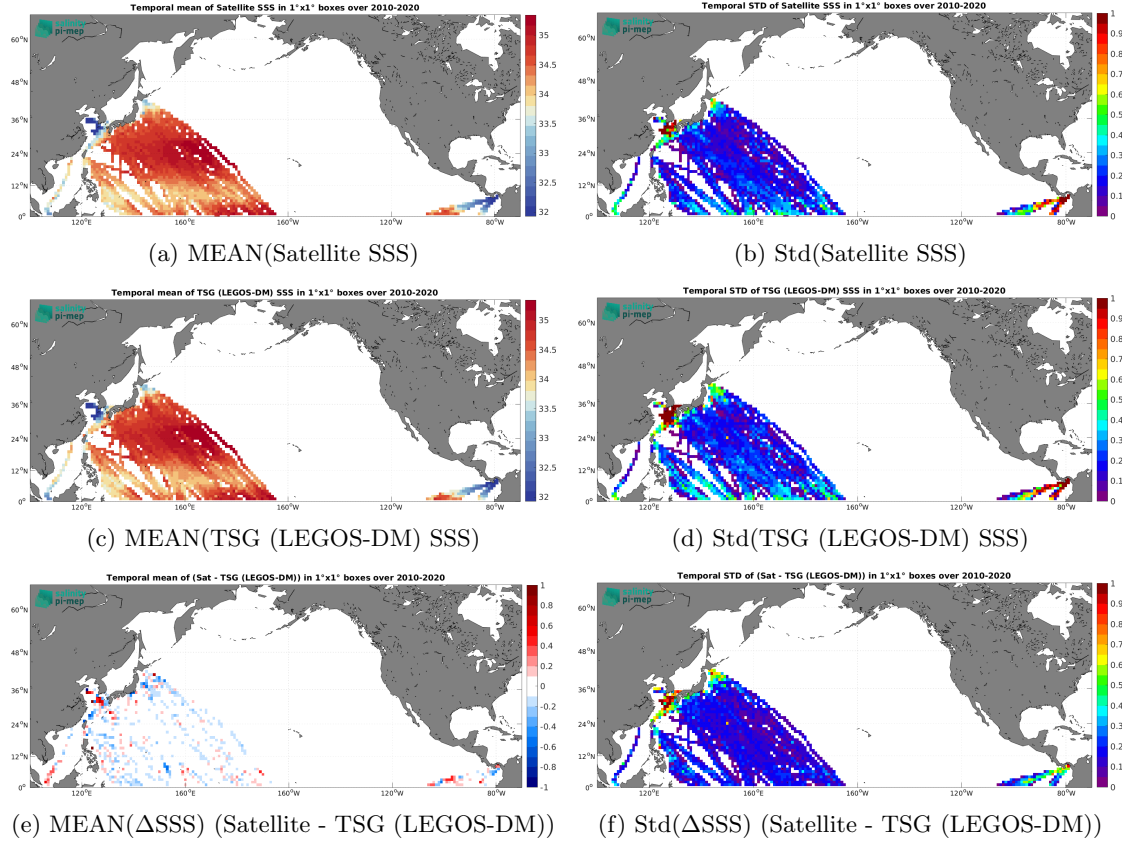
Figure 6: Temporal mean (left) and Std (right) of SSS from CCI SSS L4 Merged-OI v3.2 - 7-day running (ESA) (top), TSG (LEGOS-DM) (middle), and of \Delta\text{SSS} (Satellite - TSG (LEGOS-DM)). Only match-up pairs are used to generate these maps.
