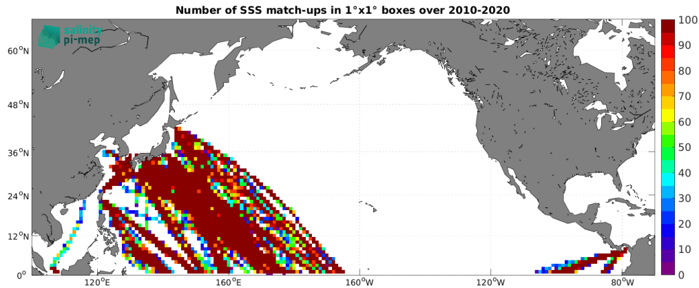
Figure 4: Number of SSS match-ups between TSG (LEGOS-DM) SSS and the CCI SSS L4 Merged-OI v3.2 - 7-day running (ESA) SSS product for the North Pacific Ocean Pi-MEP region over 1^\circ \times 1^\circ boxes and for the full satellite product period.
