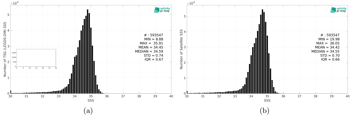
Figure 2: Histograms of SSS from TSG (LEGOS-DM) (a) and CCI SSS L4 Merged-OI v3.2 - 7-day running (ESA) (b) considering all match-up pairs per bins of 0.1 over the North Pacific Ocean Pi-MEP region and for the full satellite product period.
