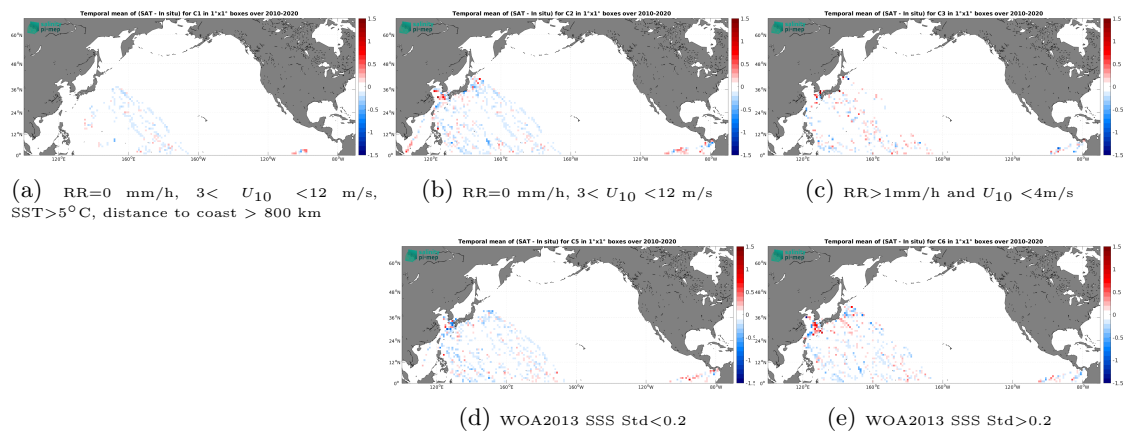
Figure 12: Temporal mean gridded over spatial boxes of size 1^\circ \times 1^\circ of \Delta\text{SSS} (CCI SSS L4 Merged-OI v3.2 - 7-day running (ESA) - TSG (LEGOS-DM)) for 5 different subdatasets corresponding to:RR=0 mm/h, 3 < U_{10} < 12 m/s, SST >5^\circ\text{C} , distance to coast > 800 km (a), RR=0 mm/h, 3 < U_{10} < 12 m/s (b), RR >1 mm/h and U_{10} < 4 m/s (c), WOA2013 SSS Std <0.2 (d), WOA2013 SSS Std >0.2 (e).
