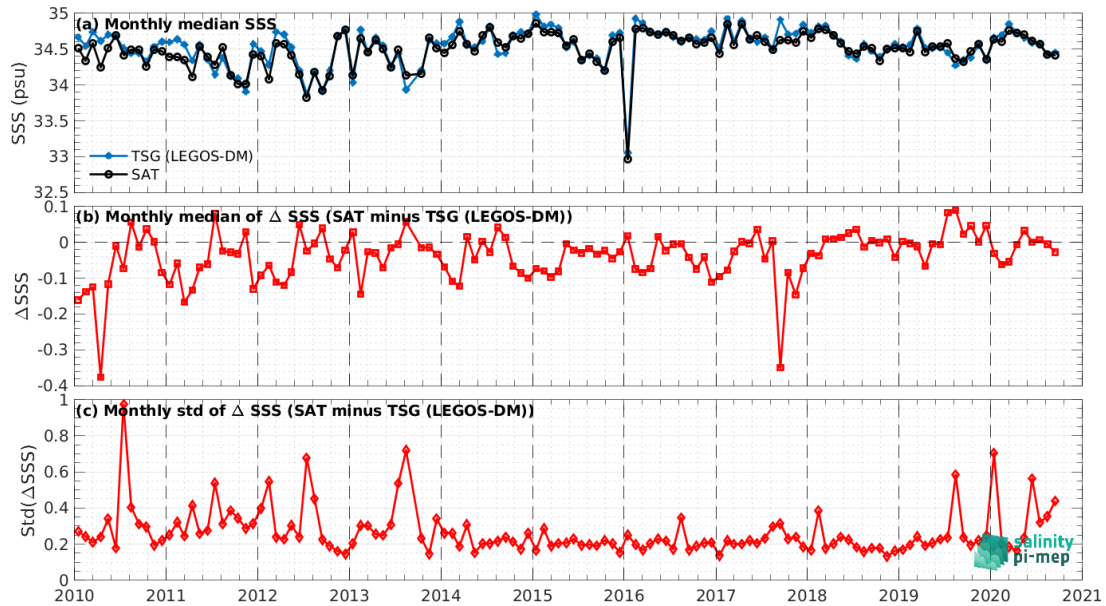
Figure 7: Time series of the monthly median SSS (top), median of \Delta\text{SSS} (Satellite - TSG (LEGOS-DM)) and Std of \Delta\text{SSS} (Satellite - TSG (LEGOS-DM)) over the North Pacific Ocean Pi-MEP region considering all match-ups collected by the Pi-MEP.
