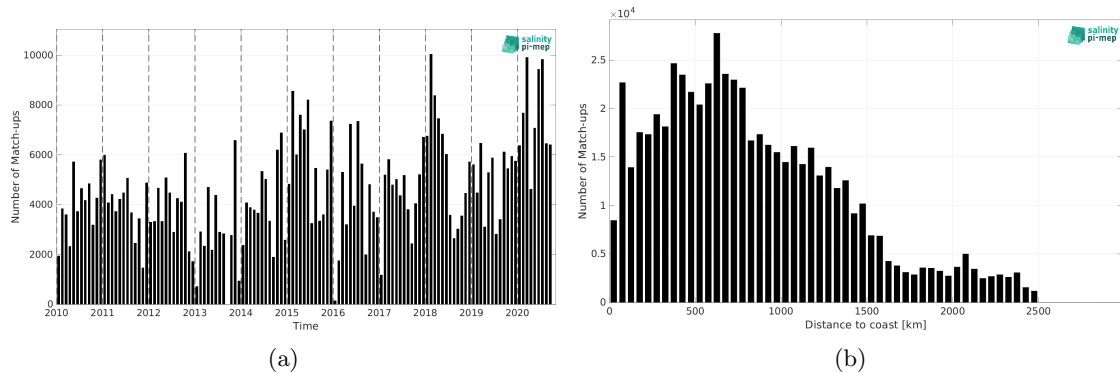
Figure 1: Number of match-ups between TSG (LEGOS-DM) and CCI SSS L4 Merged-OI v3.2 - 7-day running (ESA) SSS as a function of time (a) and as function of the distance to coast (b) over the North Pacific Ocean Pi-MEP region and for the full satellite product period.
