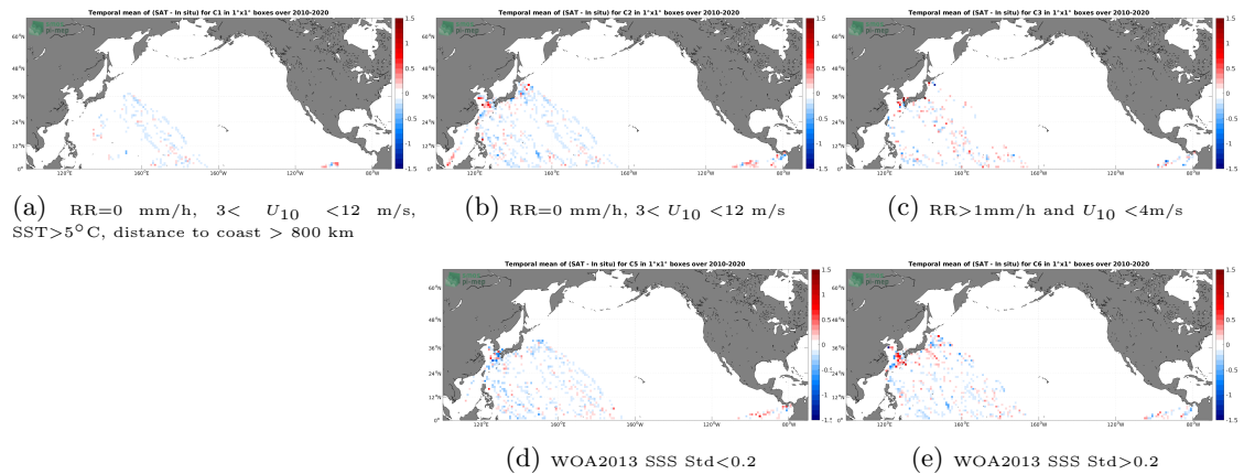
Figure 12: Temporal mean gridded over spatial boxes of size 1^\circ \times 1^\circ of \Delta SSS (CCI SSS L4 Merged-OI v3.2 - 7-day running (ESA) - TSG (LEGOS-DM)) for 5 different subdatasets corresponding to:RR=0 mm/h, 3 < U_{10} < 12 m/s, SST >5^\circ C, distance to coast > 800 km (a), RR=0 mm/h, 3 < U_{10} < 12 m/s (b), RR >1 mm/h and U_{10} < 4 m/s (c), WOA2013 SSS Std <0.2 (d), WOA2013 SSS Std >0.2 (e).
