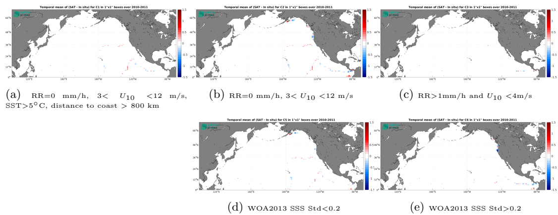
Figure 12: Temporal mean gridded over spatial boxes of size 1^\circ \times 1^\circ of \Delta\text{SSS} (CCI SSS L4 Merged-OI v3.2 - 7-day running (ESA) - TSG (GOSUD-Sailing-ship)) for 5 different subdatasets corresponding to: RR=0 mm/h, 3 < U_{10} < 12 m/s, SST > 5°C, distance to coast > 800 km (a), RR=0 mm/h, 3 < U_{10} < 12 m/s (b), RR > 1mm/h and U_{10} < 4 m/s (c), WOA2013 SSS Std < 0.2 (d), WOA2013 SSS Std > 0.2 (e).
