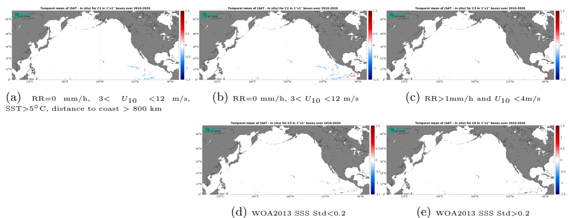
Figure 12: Temporal mean gridded over spatial boxes of size 1^\circ \times 1^\circ of \Delta\text{SSS} (CCI SSS L4 Merged-OI v3.2 - 7-day running (ESA) - TSG (GOSUD-Research-vessel)) for 5 different subdatasets corresponding to:RR=0 mm/h, 3 < U_{10} < 12 m/s, SST>5°C, distance to coast > 800 km (a), RR=0 mm/h, 3 < U_{10} < 12 m/s (b), RR>1mm/h and U_{10} < 4 m/s (c), WOA2013 SSS Std<0.2 (d), WOA2013 SSS Std>0.2 (e).
