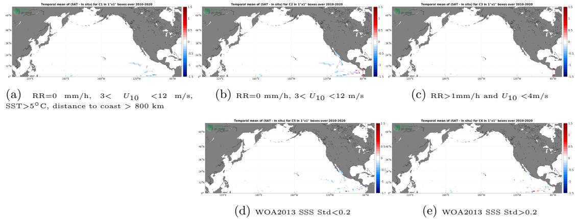
Figure 12: Temporal mean gridded over spatial boxes of size 1^\circ \times 1^\circ of \Delta SSS (CCI SSS L4 Merged-OI v3.2 - 7-day running (ESA) - TSG (GOSUD-Research-vessel)) for 5 different subdatasets corresponding to:RR=0 mm/h, 3 < U_{10} < 12 m/s, SST >5^\circ\text{C} , distance to coast > 800 km (a), RR=0 mm/h, 3 < U_{10} < 12 m/s (b), RR >1 mm/h and U_{10} < 4 m/s (c), WOA2013 SSS Std <0.2 (d), WOA2013 SSS Std >0.2 (e).
