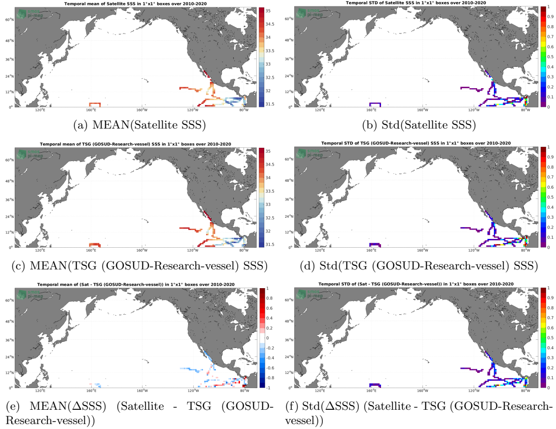
Figure 6: Temporal mean (left) and Std (right) of SSS from CCI SSS L4 Merged-OI v3.2 - 7-day running (ESA) (top), TSG (GOSUD-Research-vessel) (middle), and of \Delta SSS (Satellite - TSG (GOSUD-Research-vessel)). Only match-up pairs are used to generate these maps.
