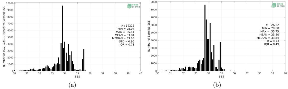
Figure 2: Histograms of SSS from TSG (GOSUD-Research-vessel) (a) and CCI SSS L4 Merged-OI v3.2 - 7-day running (ESA) (b) considering all match-up pairs per bins of 0.1 over the North Pacific Ocean Pi-MEP region and for the full satellite product period.
