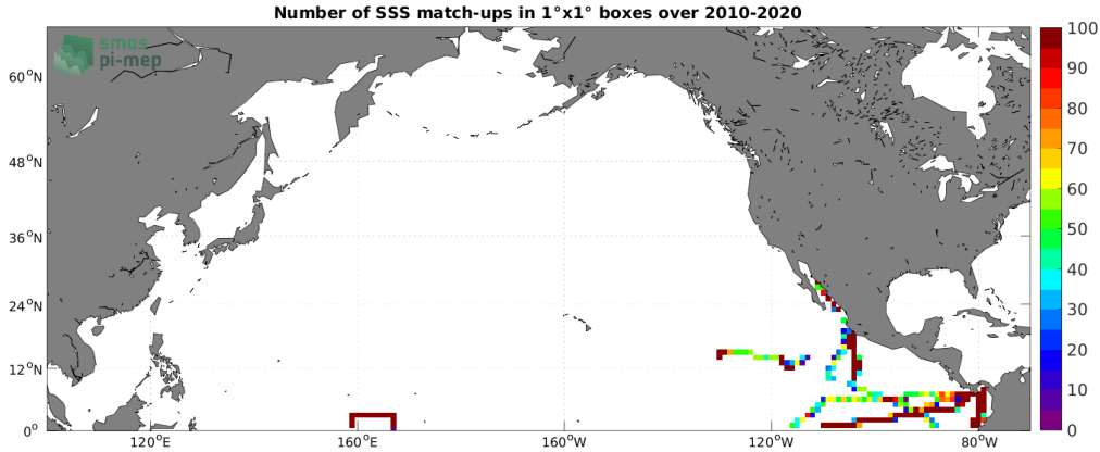
Figure 4: Number of SSS match-ups between TSG (GOSUD-Research-vessel) SSS and the CCI SSS L4 Merged-OI v3.2 - 7-day running (ESA) SSS product for the North Pacific Ocean Pi-MEP region over 1^\circ \times 1^\circ boxes and for the full satellite product period.
