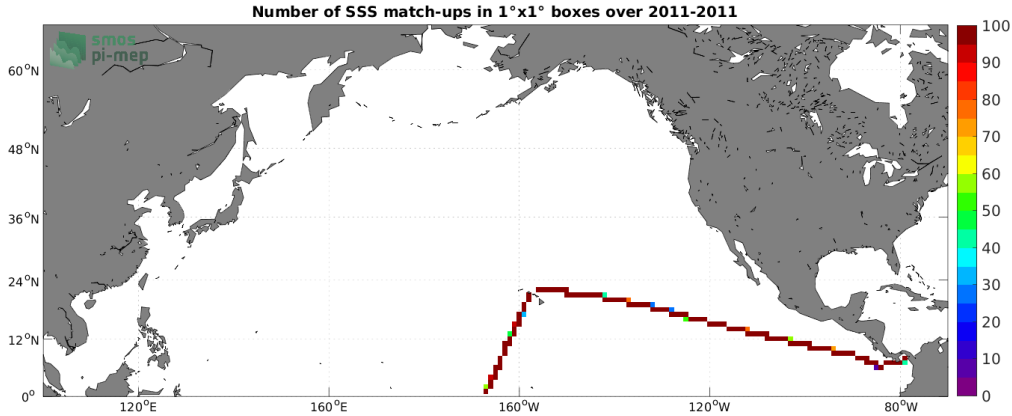
Figure 4: Number of SSS match-ups between TSG (CSIC-UTM) SSS and the CCI SSS L4 Merged-OI v3.2 - 7-day running (ESA) SSS product for the North Pacific Ocean Pi-MEP region over 1^\circ \times 1^\circ boxes and for the full satellite product period.
