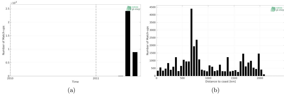
Figure 1: Number of match-ups between TSG (CSIC-UTM) and CCI SSS L4 Merged-OI v3.2 - 7-day running (ESA) SSS as a function of time (a) and as function of the distance to coast (b) over the North Pacific Ocean Pi-MEP region and for the full satellite product period.
