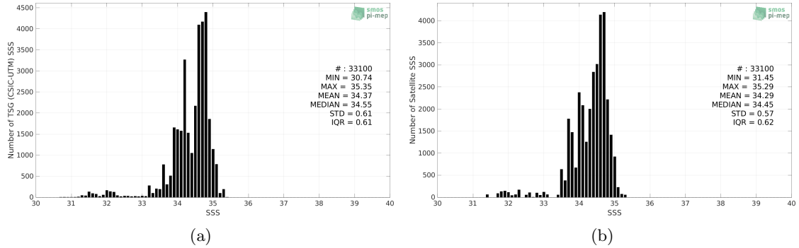
Figure 2: Histograms of SSS from TSG (CSIC-UTM) (a) and CCI SSS L4 Merged-OI v3.2 - 7-day running (ESA) (b) considering all match-up pairs per bins of 0.1 over the North Pacific Ocean Pi-MEP region and for the full satellite product period.
