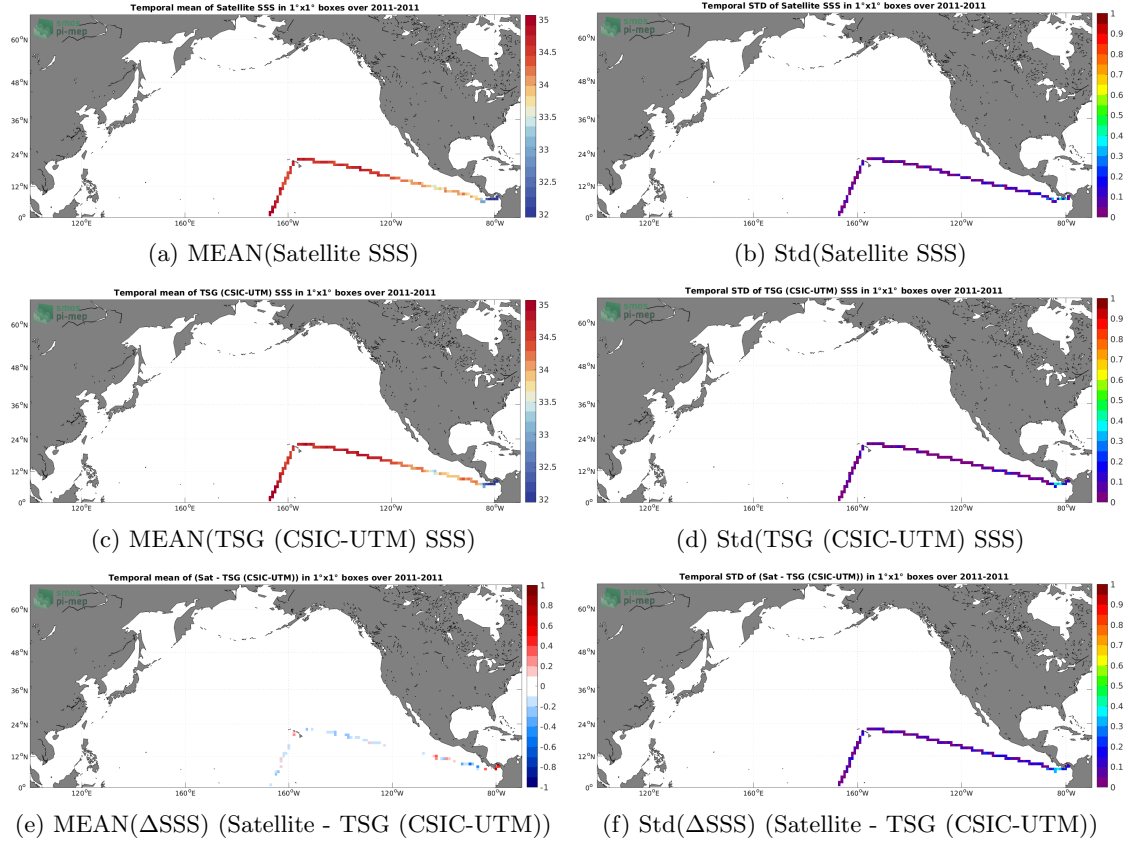
Figure 6: Temporal mean (left) and Std (right) of SSS from CCI SSS L4 Merged-OI v3.2 - 7-day running (ESA) (top), TSG (CSIC-UTM) (middle), and of \Delta SSS (Satellite - TSG (CSIC-UTM)). Only match-up pairs are used to generate these maps.
