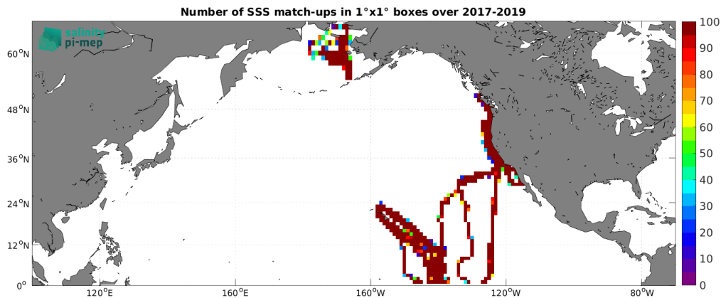
Figure 4: Number of SSS match-ups between Saildrone SSS and the CCI SSS L4 Merged-OI v3.2 - 7-day running (ESA) SSS product for the North Pacific Ocean Pi-MEP region over 1^\circ \times 1^\circ boxes and for the full satellite product period.
