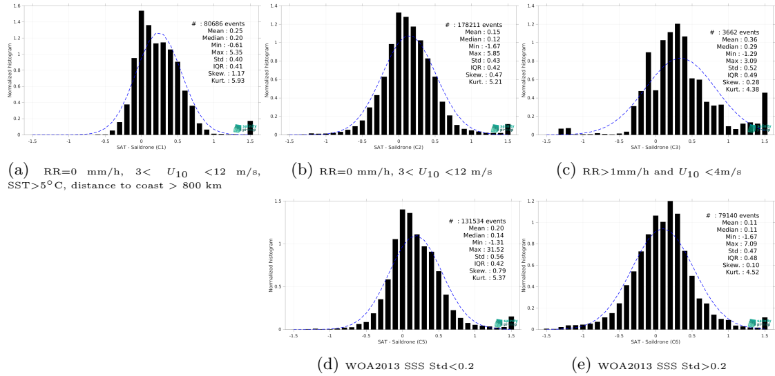
Figure 13: Normalized histogram of \Delta\text{SSS} (CCI SSS L4 Merged-OI v3.2 - 7-day running (ESA) - Sailldrone) for 5 different subdatasets corresponding to: RR=0 mm/h, 3 < U_{10} < 12 m/s, SST>5°C, distance to coast > 800 km (a), RR=0 mm/h, 3 < U_{10} < 12 m/s (b), RR>1mm/h and U_{10} < 4 m/s (c), WOA2013 SSS Std<0.2 (d), WOA2013 SSS Std>0.2 (e).
