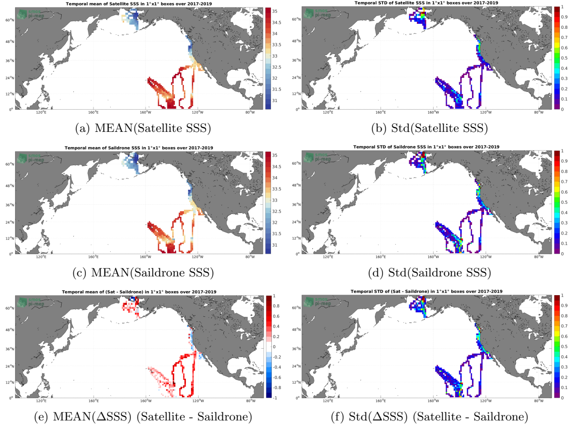
Figure 6: Temporal mean (left) and Std (right) of SSS from CCI SSS L4 Merged-OI v3.2 - 7-day running (ESA) (top), Saildrone (middle), and of \Delta\text{SSS} (Satellite - Saildrone). Only match-up pairs are used to generate these maps.
