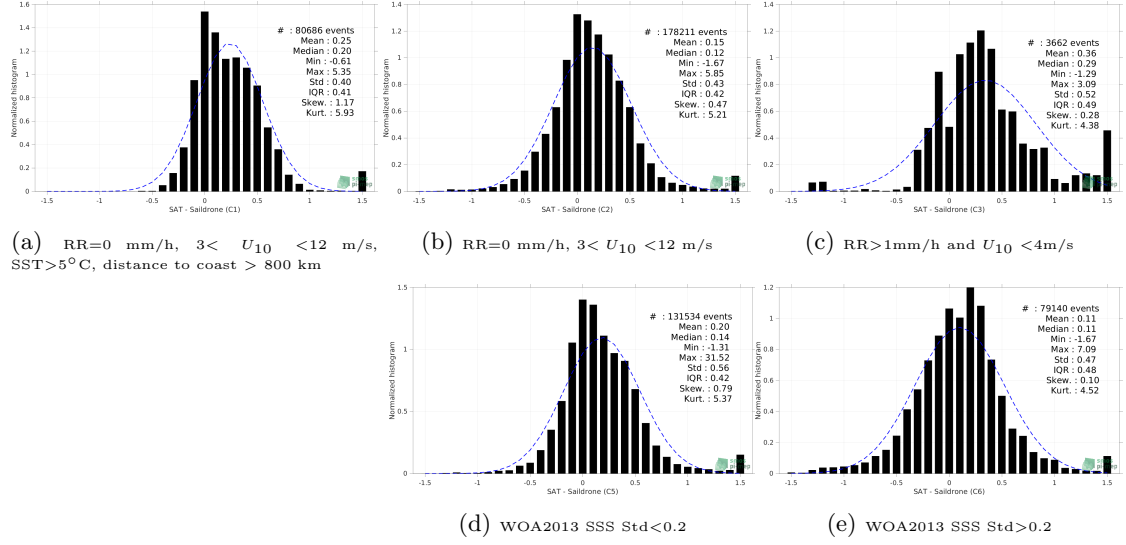
Figure 13: Normalized histogram of \Delta SSS (CCI SSS L4 Merged-OI v3.2 - 7-day running (ESA) - Sailldrone) for 5 different subdatasets corresponding to: RR=0 mm/h, 3 < U_{10} < 12 m/s, SST>5°C, distance to coast > 800 km (a), RR=0 mm/h, 3 < U_{10} < 12 m/s (b), RR>1mm/h and U_{10} < 4 m/s (c), WOA2013 SSS Std<0.2 (d), WOA2013 SSS Std>0.2 (e).
