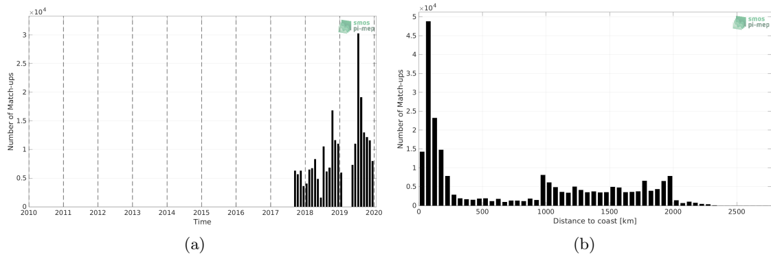
Figure 1: Number of match-ups between Saildrone and CCI SSS L4 Merged-OI v3.2 - 7-day running (ESA) SSS as a function of time (a) and as function of the distance to coast (b) over the North Pacific Ocean Pi-MEP region and for the full satellite product period.
