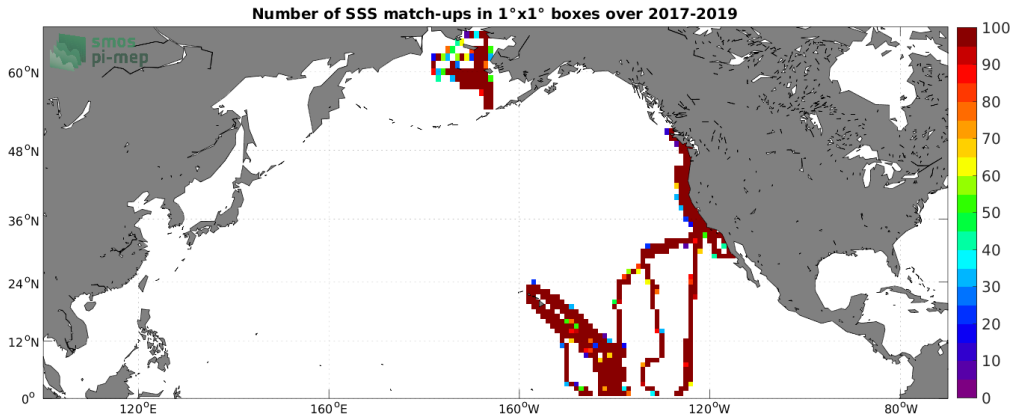
Figure 4: Number of SSS match-ups between Sailldrone SSS and the CCI SSS L4 Merged-OI v3.2 - 7-day running (ESA) SSS product for the North Pacific Ocean Pi-MEP region over 1^\circ \times 1^\circ boxes and for the full satellite product period.
