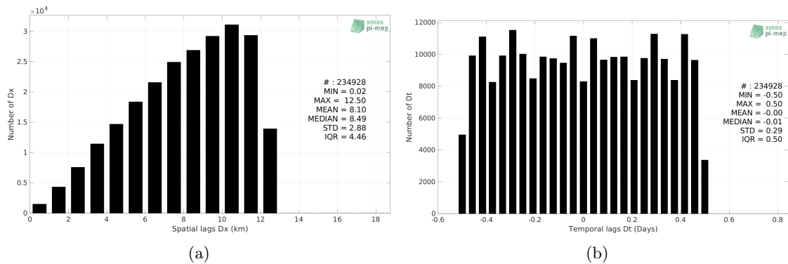
Figure 5: Histograms of the spatial (a) and temporal (b) lags between the location/time of the Sailldrone measurement and the date of the corresponding CCI SSS L4 Merged-OI v3.2 - 7-day running (ESA) SSS pixel.
