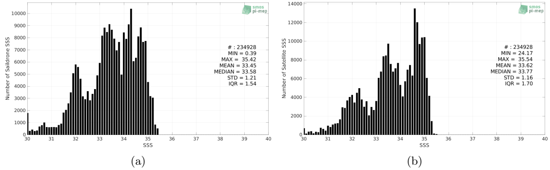
Figure 2: Histograms of SSS from Saildrone (a) and CCI SSS L4 Merged-OI v3.2 - 7-day running (ESA) (b) considering all match-up pairs per bins of 0.1 over the North Pacific Ocean Pi-MEP region and for the full satellite product period.
