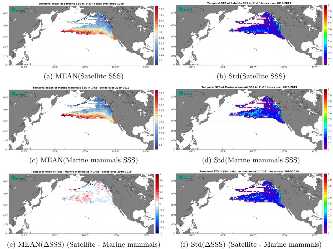
Figure 6: Temporal mean (left) and Std (right) of SSS from CCI SSS L4 Merged-OI v3.2 - 7-day running (ESA) (top), Marine mammals (middle), and of \Delta SSS (Satellite - Marine mammals). Only match-up pairs are used to generate these maps.
