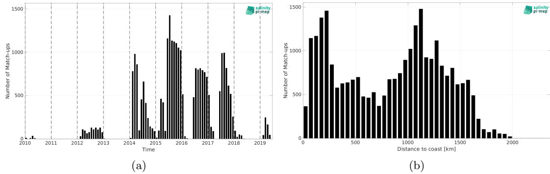
Figure 1: Number of match-ups between Marine mammals and CCI SSS L4 Merged-OI v3.2 - 7-day running (ESA) SSS as a function of time (a) and as function of the distance to coast (b) over the North Pacific Ocean Pi-MEP region and for the full satellite product period.
