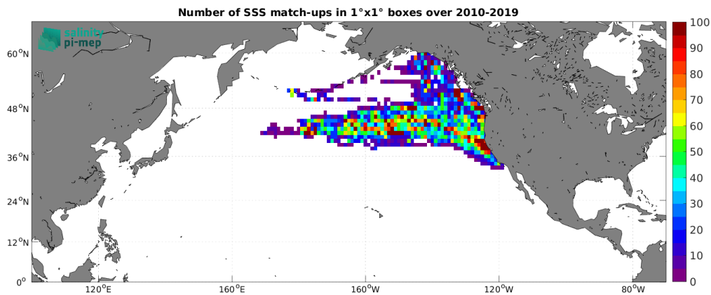
Figure 4: Number of SSS match-ups between Marine mammals SSS and the CCI SSS L4 Merged-OI v3.2 - 7-day running (ESA) SSS product for the North Pacific Ocean Pi-MEP region over 1^\circ \times 1^\circ boxes and for the full satellite product period.
