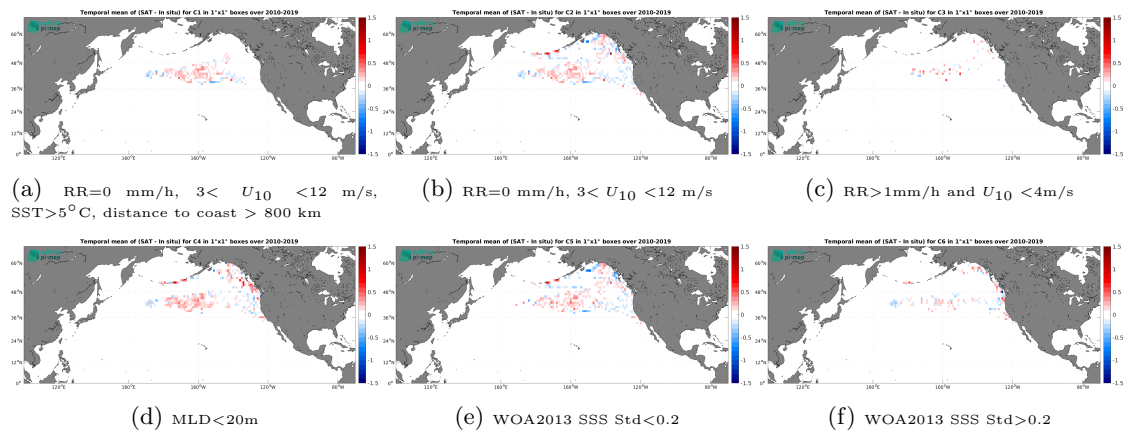
Figure 12: Temporal mean gridded over spatial boxes of size 1^\circ \times 1^\circ of \Delta SSS (CCI SSS L4 Merged-OI v3.2 - 7-day running (ESA) - Marine mammals) for 6 different subdatasets corresponding to:RR=0 mm/h, 3 < U_{10} < 12 m/s, SST >5^\circ C, distance to coast > 800 km (a), RR=0 mm/h, 3 < U_{10} < 12 m/s (b), RR >1 mm/h and U_{10} < 4 m/s (c),MLD <20 m (d),WOA2013 SSS Std <0.2 (e),WOA2013 SSS Std >0.2 (f).
