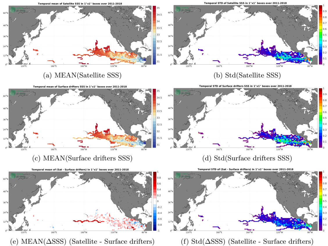
Figure 5: Temporal mean (left) and Std (right) of SSS from CCI SSS L4 Merged-OI v3.2 - 7-day running (ESA) (top), Surface drifters (middle), and of \Delta SSS (Satellite - Surface drifters). Only match-up pairs are used to generate these maps.
