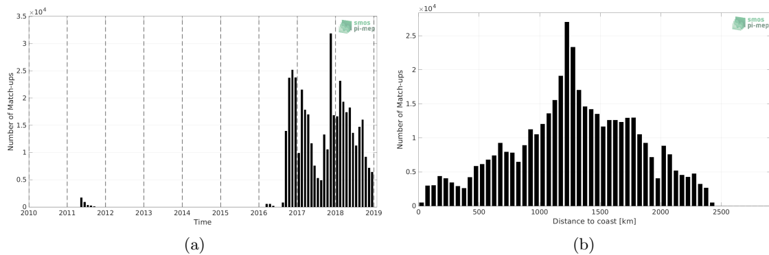
Figure 1: Number of match-ups between Surface drifters and CCI SSS L4 Merged-OI v3.2 - 7-day running (ESA) SSS as a function of time (a) and as function of the distance to coast (b) over the North Pacific Ocean Pi-MEP region and for the full satellite product period.
