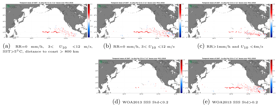
Figure 11: Temporal mean gridded over spatial boxes of size 1^\circ \times 1^\circ of \Delta SSS (CCI SSS L4 Merged-OI v3.2 - 7-day running (ESA) - Surface drifters) for 5 different subdatasets corresponding to:RR=0 mm/h, 3 < U_{10} < 12 m/s, SST >5^\circ C, distance to coast > 800 km (a), RR=0 mm/h, 3 < U_{10} < 12 m/s (b), RR >1 mm/h and U_{10} < 4 m/s (c), WOA2013 SSS Std <0.2 (d), WOA2013 SSS Std >0.2 (e).
