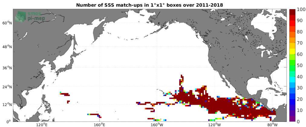
Figure 3: Number of SSS match-ups between Surface drifters SSS and the CCI SSS L4 Merged-OI v3.2 - 7-day running (ESA) SSS product for the North Pacific Ocean Pi-MEP region over 1^\circ \times 1^\circ boxes and for the full satellite product period.
