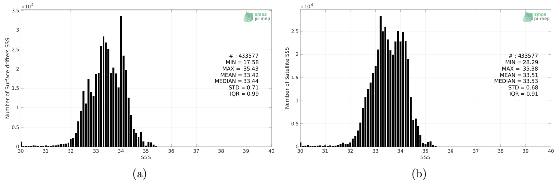
Figure 2: Histograms of SSS from Surface drifters (a) and CCI SSS L4 Merged-OI v3.2 - 7-day running (ESA) (b) considering all match-up pairs per bins of 0.1 over the North Pacific Ocean Pi-MEP region and for the full satellite product period.
