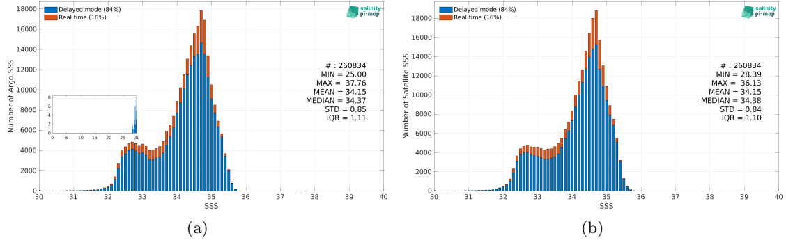
Figure 2: Histograms of SSS from Argo (a) and CCI SSS L4 Merged-OI v3.2 - 7-day running (ESA) (b) considering all match-up pairs per bins of 0.1 over the North Pacific Ocean Pi-MEP region and for the full satellite product period.
