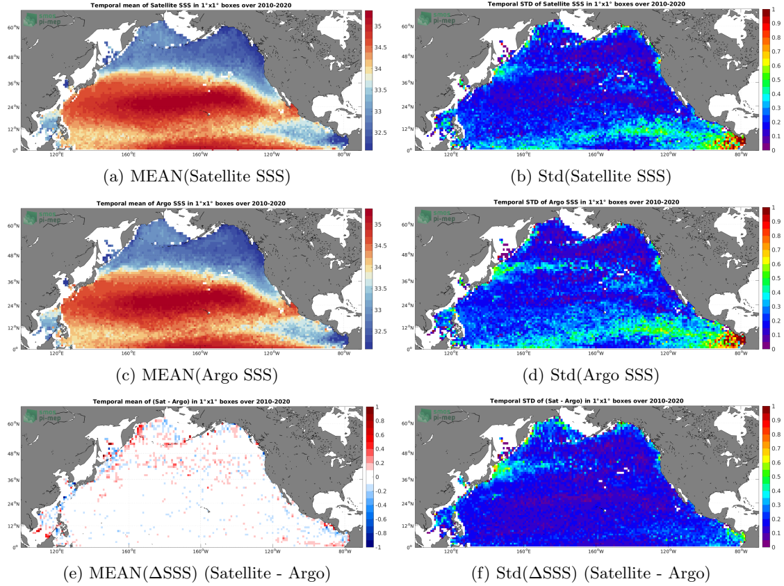
Figure 6: Temporal mean (left) and Std (right) of SSS from CCI SSS L4 Merged-OI v3.2 - 7-day running (ESA) (top), Argo (middle), and of \Delta\text{SSS} (Satellite - Argo). Only match-up pairs are used to generate these maps.
