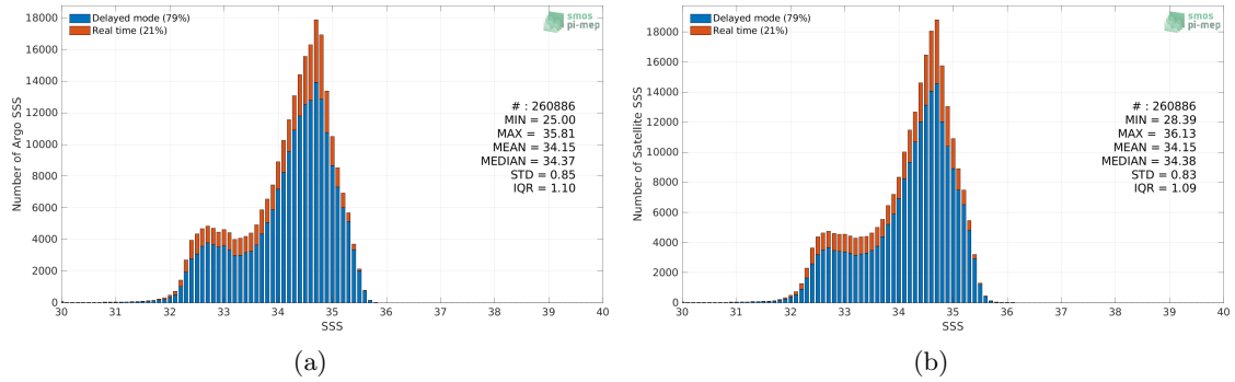
Figure 2: Histograms of SSS from Argo (a) and CCI SSS L4 Merged-OI v3.2 - 7-day running (ESA) (b) considering all match-up pairs per bins of 0.1 over the North Pacific Ocean Pi-MEP region and for the full satellite product period.
