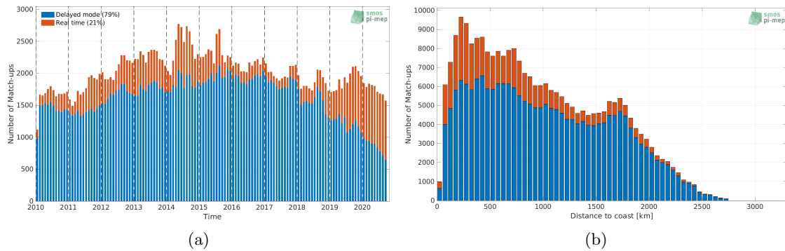
Figure 1: Number of match-ups between Argo and CCI SSS L4 Merged-OI v3.2 - 7-day running (ESA) SSS as a function of time (a) and as function of the distance to coast (b) over the North Pacific Ocean Pi-MEP region and for the full satellite product period.
