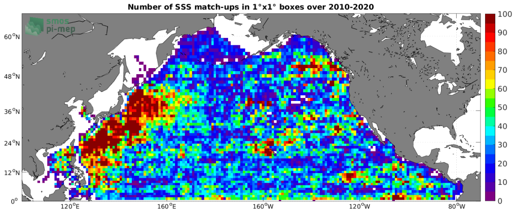
Figure 4: Number of SSS match-ups between Argo SSS and the CCI SSS L4 Merged-OI v3.2 - 7-day running (ESA) SSS product for the North Pacific Ocean Pi-MEP region over 1^\circ \times 1^\circ boxes and for the full satellite product period.
