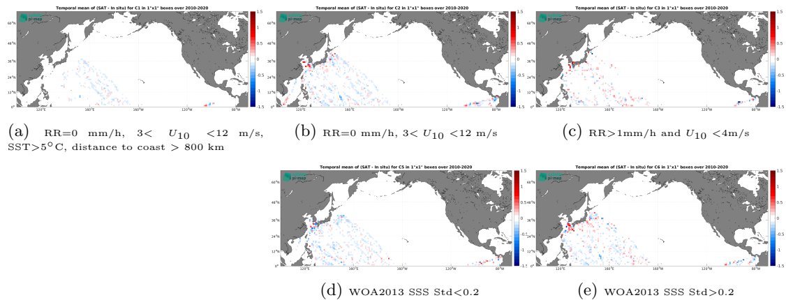
Figure 12: Temporal mean gridded over spatial boxes of size 1^\circ \times 1^\circ of \Delta\text{SSS} (CCI SSS L4 Merged-OI v3.2 - 30-day running (ESA) - TSG (LEGOS-DM)) for 5 different subdatasets corresponding to:RR=0 mm/h, 3 < U_{10} < 12 m/s, SST >5^\circ\text{C} , distance to coast > 800 km (a), RR=0 mm/h, 3 < U_{10} < 12 m/s (b), RR >1 mm/h and U_{10} < 4 m/s (c), WOA2013 SSS Std <0.2 (d), WOA2013 SSS Std >0.2 (e).
