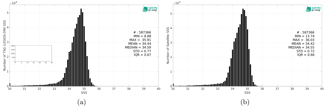
Figure 2: Histograms of SSS from TSG (LEGOS-DM) (a) and CCI SSS L4 Merged-OI v3.2 - 30-day running (ESA) (b) considering all match-up pairs per bins of 0.1 over the North Pacific Ocean Pi-MEP region and for the full satellite product period.
