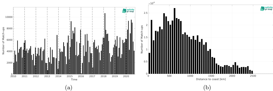
Figure 1: Number of match-ups between TSG (LEGOS-DM) and CCI SSS L4 Merged-OI v3.2 - 30-day running (ESA) SSS as a function of time (a) and as function of the distance to coast (b) over the North Pacific Ocean Pi-MEP region and for the full satellite product period.
