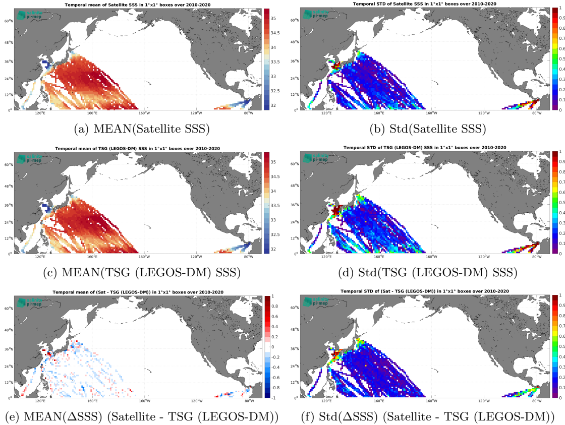
Figure 6: Temporal mean (left) and Std (right) of SSS from CCI SSS L4 Merged-OI v3.2 - 30-day running (ESA) (top), TSG (LEGOS-DM) (middle), and of \Delta\text{SSS} (Satellite - TSG (LEGOS-DM)). Only match-up pairs are used to generate these maps.
