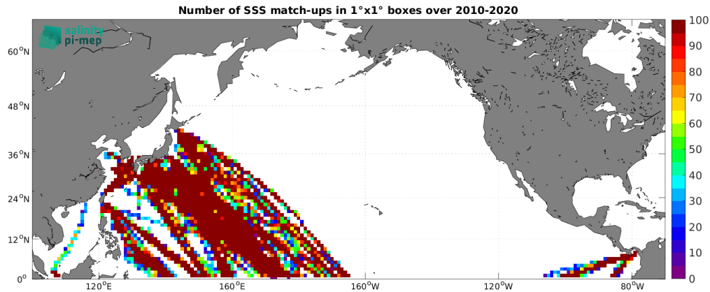
Figure 4: Number of SSS match-ups between TSG (LEGOS-DM) SSS and the CCI SSS L4 Merged-OI v3.2 - 30-day running (ESA) SSS product for the North Pacific Ocean Pi-MEP region over 1^\circ \times 1^\circ boxes and for the full satellite product period.
