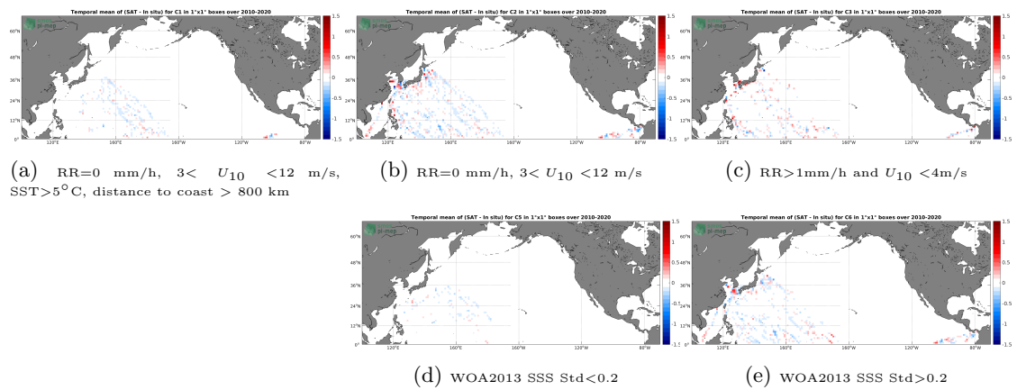
Figure 12: Temporal mean gridded over spatial boxes of size 1^\circ \times 1^\circ of \Delta SSS (CCI SSS L4 Merged-OI v3.2 - 30-day running (ESA) - TSG (LEGOS-DM)) for 5 different subdatasets corresponding to:RR=0 mm/h, 3 < U_{10} < 12 m/s, SST >5^\circ\text{C} , distance to coast > 800 km (a), RR=0 mm/h, 3 < U_{10} < 12 m/s (b), RR >1 mm/h and U_{10} < 4 m/s (c), WOA2013 SSS Std <0.2 (d), WOA2013 SSS Std >0.2 (e).
