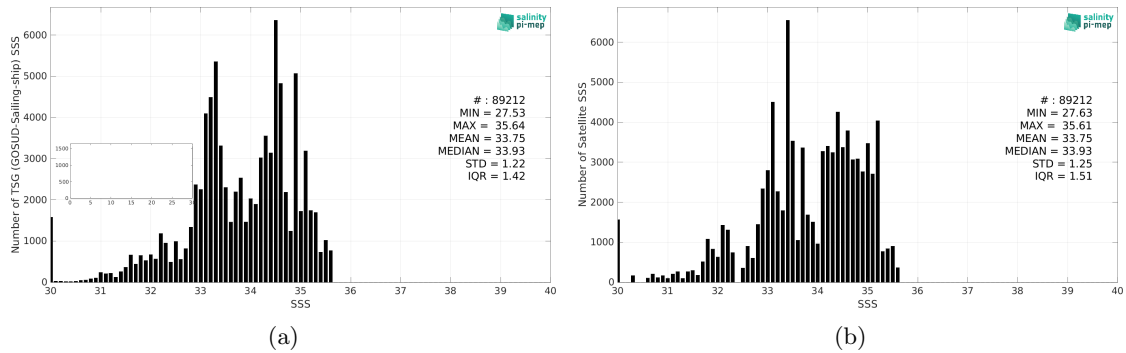
Figure 2: Histograms of SSS from TSG (GOSUD-Sailing-ship) (a) and CCI SSS L4 Merged-OI v3.2 - 30-day running (ESA) (b) considering all match-up pairs per bins of 0.1 over the North Pacific Ocean Pi-MEP region and for the full satellite product period.
