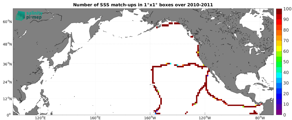
Figure 4: Number of SSS match-ups between TSG (GOSUD-Sailing-ship) SSS and the CCI SSS L4 Merged-OI v3.2 - 30-day running (ESA) SSS product for the North Pacific Ocean Pi-MEP region over 1^\circ \times 1^\circ boxes and for the full satellite product period.
