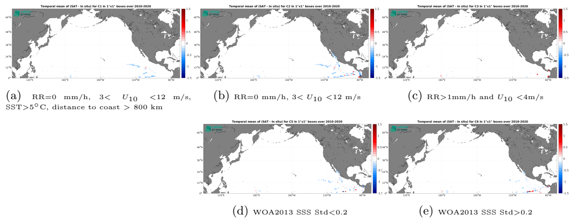
Figure 12: Temporal mean gridded over spatial boxes of size 1^\circ \times 1^\circ of \Delta\text{SSS} (CCI SSS L4 Merged-OI v3.2 - 30-day running (ESA) - TSG (GOSUD-Research-vessel)) for 5 different subdatasets corresponding to: RR=0 mm/h, 3 < U_{10} < 12 m/s, SST > 5°C, distance to coast > 800 km (a), RR=0 mm/h, 3 < U_{10} < 12 m/s (b), RR > 1mm/h and U_{10} < 4 m/s (c), WOA2013 SSS Std < 0.2 (d), WOA2013 SSS Std > 0.2 (e).
