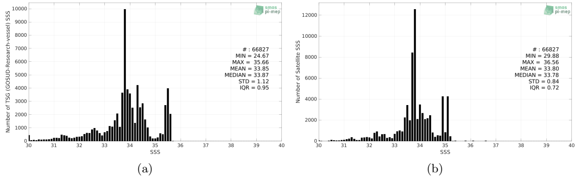
Figure 2: Histograms of SSS from TSG (GOSUD-Research-vessel) (a) and CCI SSS L4 Merged-OI v3.2 - 30-day running (ESA) (b) considering all match-up pairs per bins of 0.1 over the North Pacific Ocean Pi-MEP region and for the full satellite product period.
