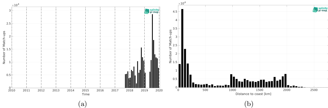
Figure 1: Number of match-ups between Saildrone and CCI SSS L4 Merged-OI v3.2 - 30-day running (ESA) SSS as a function of time (a) and as function of the distance to coast (b) over the North Pacific Ocean Pi-MEP region and for the full satellite product period.
