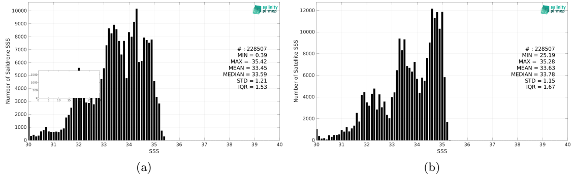
Figure 2: Histograms of SSS from Saildrone (a) and CCI SSS L4 Merged-OI v3.2 - 30-day running (ESA) (b) considering all match-up pairs per bins of 0.1 over the North Pacific Ocean Pi-MEP region and for the full satellite product period.
