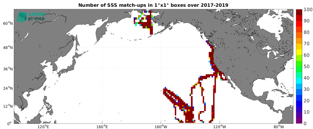
Figure 4: Number of SSS match-ups between Saildrone SSS and the CCI SSS L4 Merged-OI v3.2 - 30-day running (ESA) SSS product for the North Pacific Ocean Pi-MEP region over 1^\circ \times 1^\circ boxes and for the full satellite product period.
