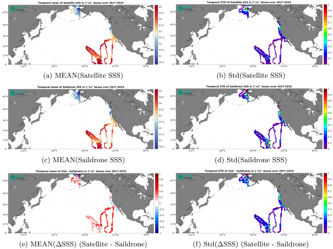
Figure 6: Temporal mean (left) and Std (right) of SSS from CCI SSS L4 Merged-OI v3.2 - 30-day running (ESA) (top), Saildrone (middle), and of \Delta\text{SSS} (Satellite - Saildrone). Only match-up pairs are used to generate these maps.
