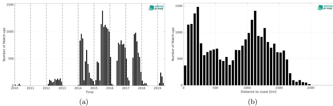
Figure 1: Number of match-ups between Marine mammals and CCI SSS L4 Merged-OI v3.2 - 30-day running (ESA) SSS as a function of time (a) and as function of the distance to coast (b) over the North Pacific Ocean Pi-MEP region and for the full satellite product period.
