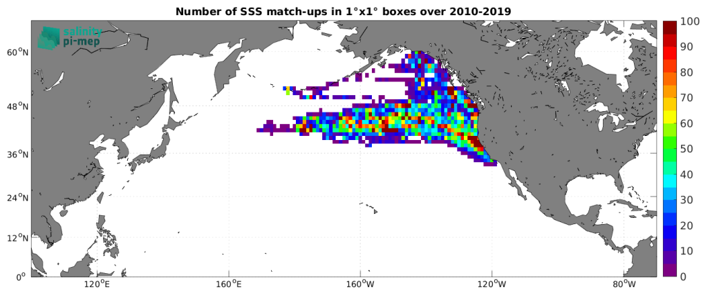
Figure 4: Number of SSS match-ups between Marine mammals SSS and the CCI SSS L4 Merged-OI v3.2 - 30-day running (ESA) SSS product for the North Pacific Ocean Pi-MEP region over 1^\circ \times 1^\circ boxes and for the full satellite product period.
