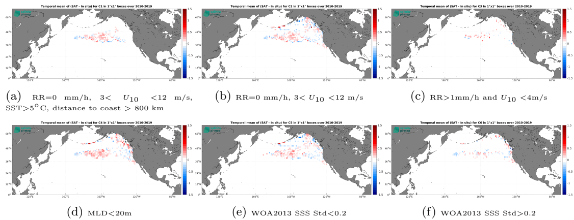
Figure 12: Temporal mean gridded over spatial boxes of size 1^\circ \times 1^\circ of \Delta SSS (CCI SSS L4 Merged-OI v3.2 - 30-day running (ESA) - Marine mammals) for 6 different subdatasets corresponding to:RR=0 mm/h, 3 < U_{10} < 12 m/s, SST >5^\circ C, distance to coast > 800 km (a), RR=0 mm/h, 3 < U_{10} < 12 m/s (b), RR >1 mm/h and U_{10} < 4 m/s (c),MLD <20 m (d),WOA2013 SSS Std <0.2 (e),WOA2013 SSS Std >0.2 (f).
