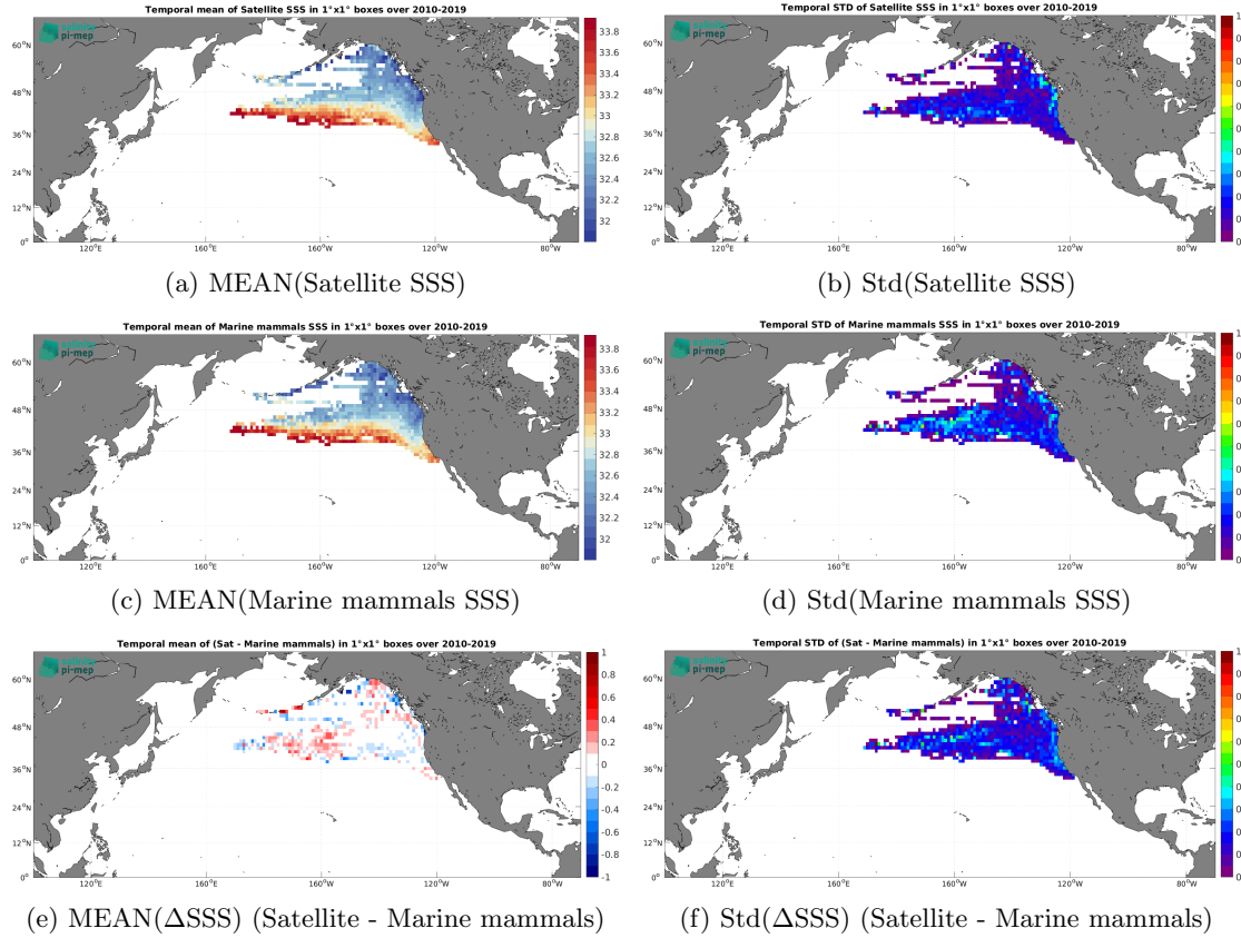
Figure 6: Temporal mean (left) and Std (right) of SSS from CCI SSS L4 Merged-OI v3.2 - 30-day running (ESA) (top), Marine mammals (middle), and of \Delta SSS (Satellite - Marine mammals). Only match-up pairs are used to generate these maps.
