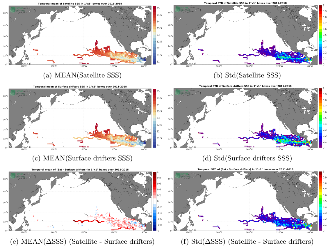
Figure 5: Temporal mean (left) and Std (right) of SSS from CCI SSS L4 Merged-OI v3.2 - 30-day running (ESA) (top), Surface drifters (middle), and of \Delta SSS (Satellite - Surface drifters). Only match-up pairs are used to generate these maps.
