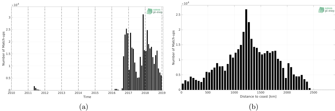
Figure 1: Number of match-ups between Surface drifters and CCI SSS L4 Merged-OI v3.2 - 30-day running (ESA) SSS as a function of time (a) and as function of the distance to coast (b) over the North Pacific Ocean Pi-MEP region and for the full satellite product period.
