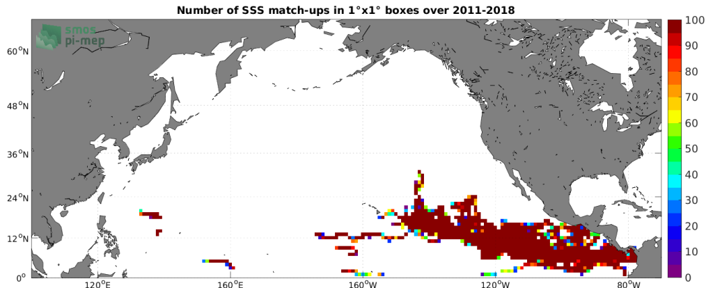
Figure 3: Number of SSS match-ups between Surface drifters SSS and the CCI SSS L4 Merged-OI v3.2 - 30-day running (ESA) SSS product for the North Pacific Ocean Pi-MEP region over 1^\circ \times 1^\circ boxes and for the full satellite product period.
