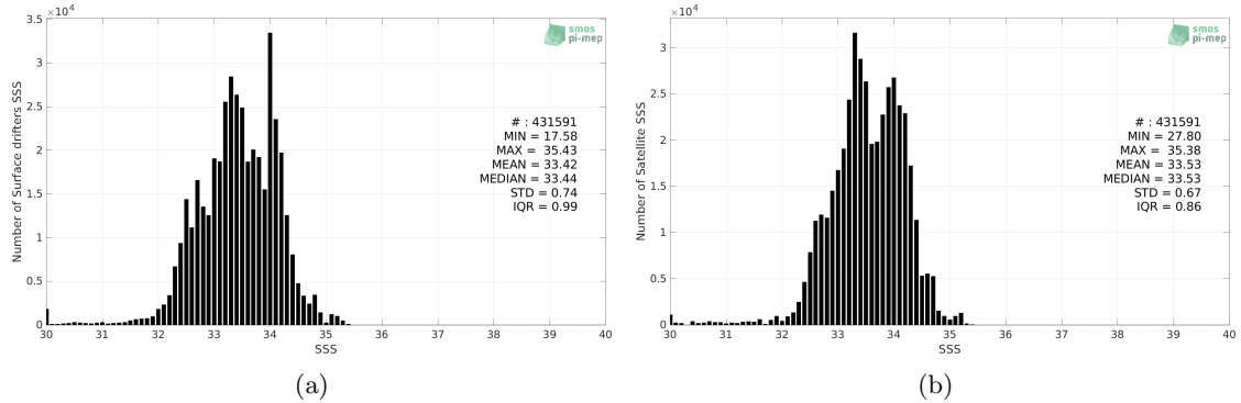
Figure 2: Histograms of SSS from Surface drifters (a) and CCI SSS L4 Merged-OI v3.2 - 30-day running (ESA) (b) considering all match-up pairs per bins of 0.1 over the North Pacific Ocean Pi-MEP region and for the full satellite product period.
