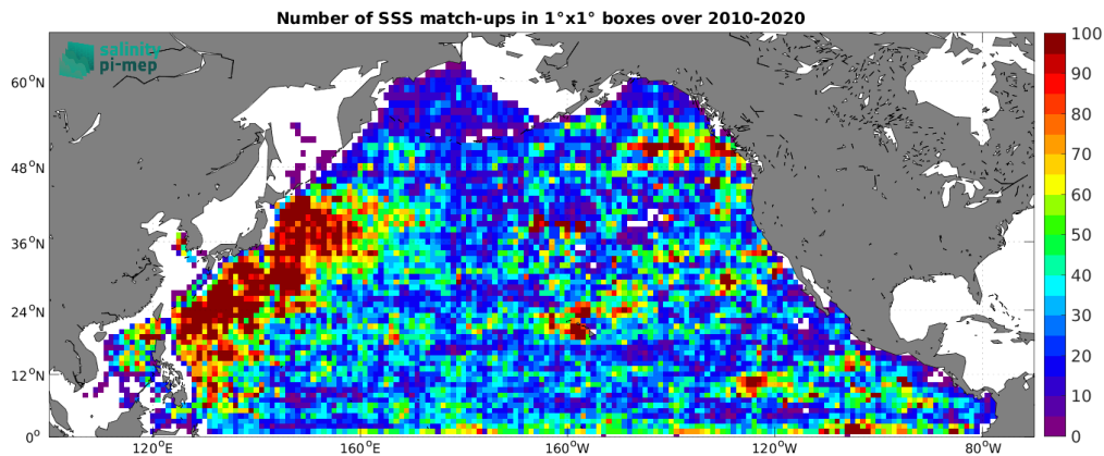
Figure 4: Number of SSS match-ups between Argo SSS and the CCI SSS L4 Merged-OI v3.2 - 30-day running (ESA) SSS product for the North Pacific Ocean Pi-MEP region over 1^\circ \times 1^\circ boxes and for the full satellite product period.
