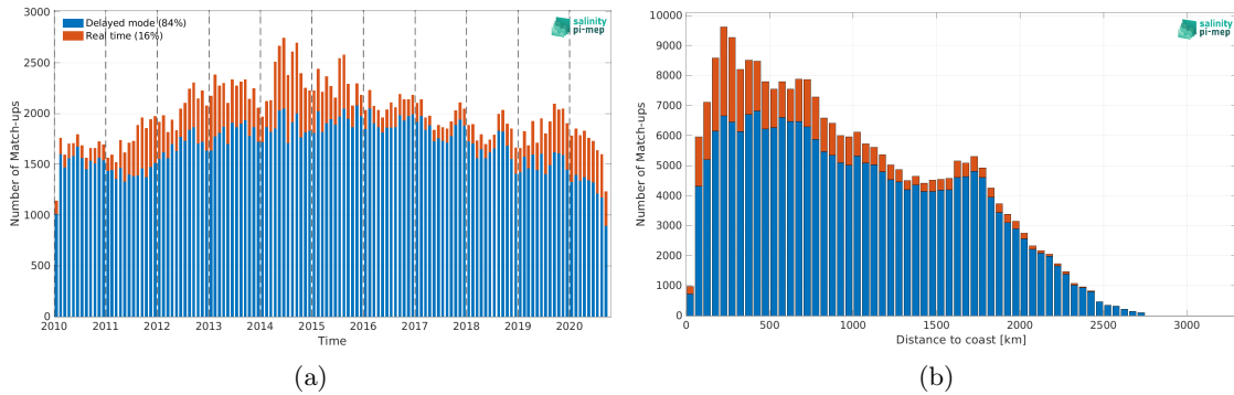
Figure 1: Number of match-ups between Argo and CCI SSS L4 Merged-OI v3.2 - 30-day running (ESA) SSS as a function of time (a) and as function of the distance to coast (b) over the North Pacific Ocean Pi-MEP region and for the full satellite product period.
