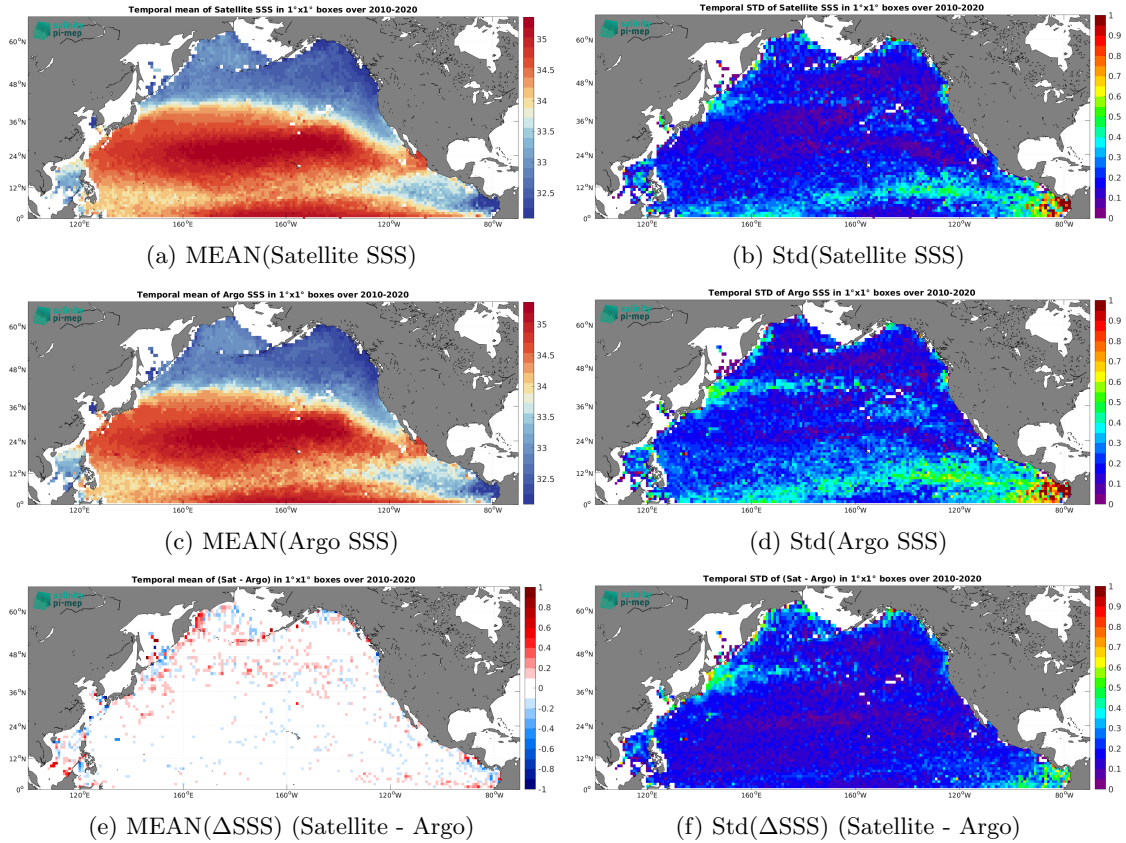
Figure 6: Temporal mean (left) and Std (right) of SSS from CCI SSS L4 Merged-OI v3.2 - 30-day running (ESA) (top), Argo (middle), and of \Delta\text{SSS} (Satellite - Argo). Only match-up pairs are used to generate these maps.
