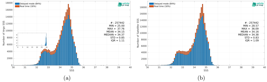
Figure 2: Histograms of SSS from Argo (a) and CCI SSS L4 Merged-OI v3.2 - 30-day running (ESA) (b) considering all match-up pairs per bins of 0.1 over the North Pacific Ocean Pi-MEP region and for the full satellite product period.
